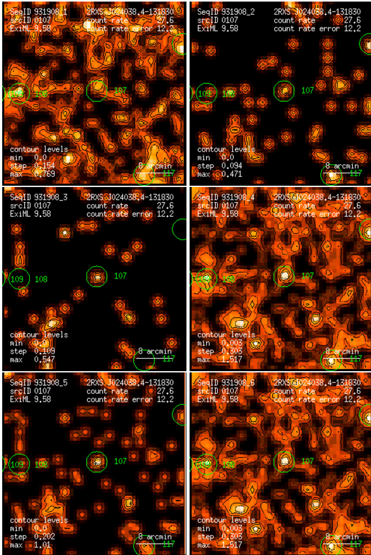
Figure 107: RASS 931908: detection 0107: band rate images, Gaussian filter: (1) PSPC channels 11 – 41, (2) 52 – 90, (3) 91 – 201, (4) 11 – 235, (5) 52 – 201, (6) 11 – 201. Broad band rates in counts/ks. Band rate contour levels in counts/ks/arcmin 2 .
