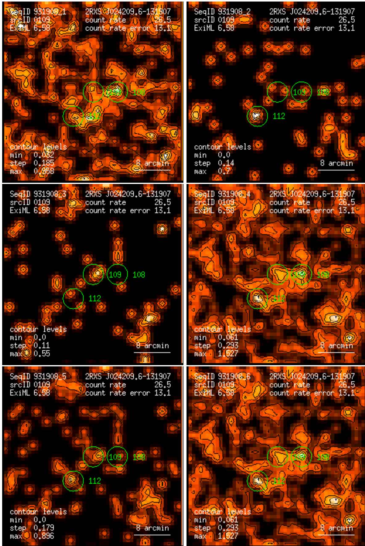
Figure 109: RASS 931908: detection 0109: band rate images, Gaussian filter: (1) PSPC channels 11 – 41, (2) 52 – 90, (3) 91 – 201, (4) 11 – 235, (5) 52 – 201, (6) 11 – 201. Broad band rates in counts/ks. Band rate contour levels in counts/ks/arcmin 2 .
