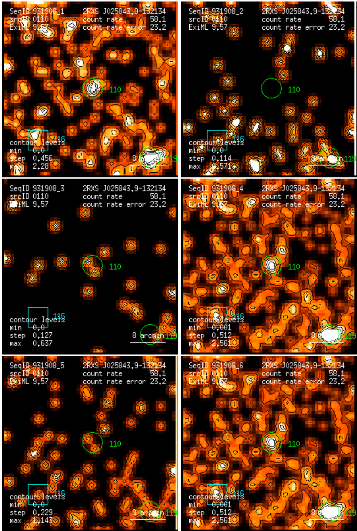
Figure 110: RASS 931908: detection 0110: band rate images, Gaussian filter: (1) PSPC channels 11 – 41, (2) 52 – 90, (3) 91 – 201, (4) 11 – 235, (5) 52 – 201, (6) 11 – 201. Broad band rates in counts/ks. Band rate contour levels in counts/ks/arcmin 2 .
