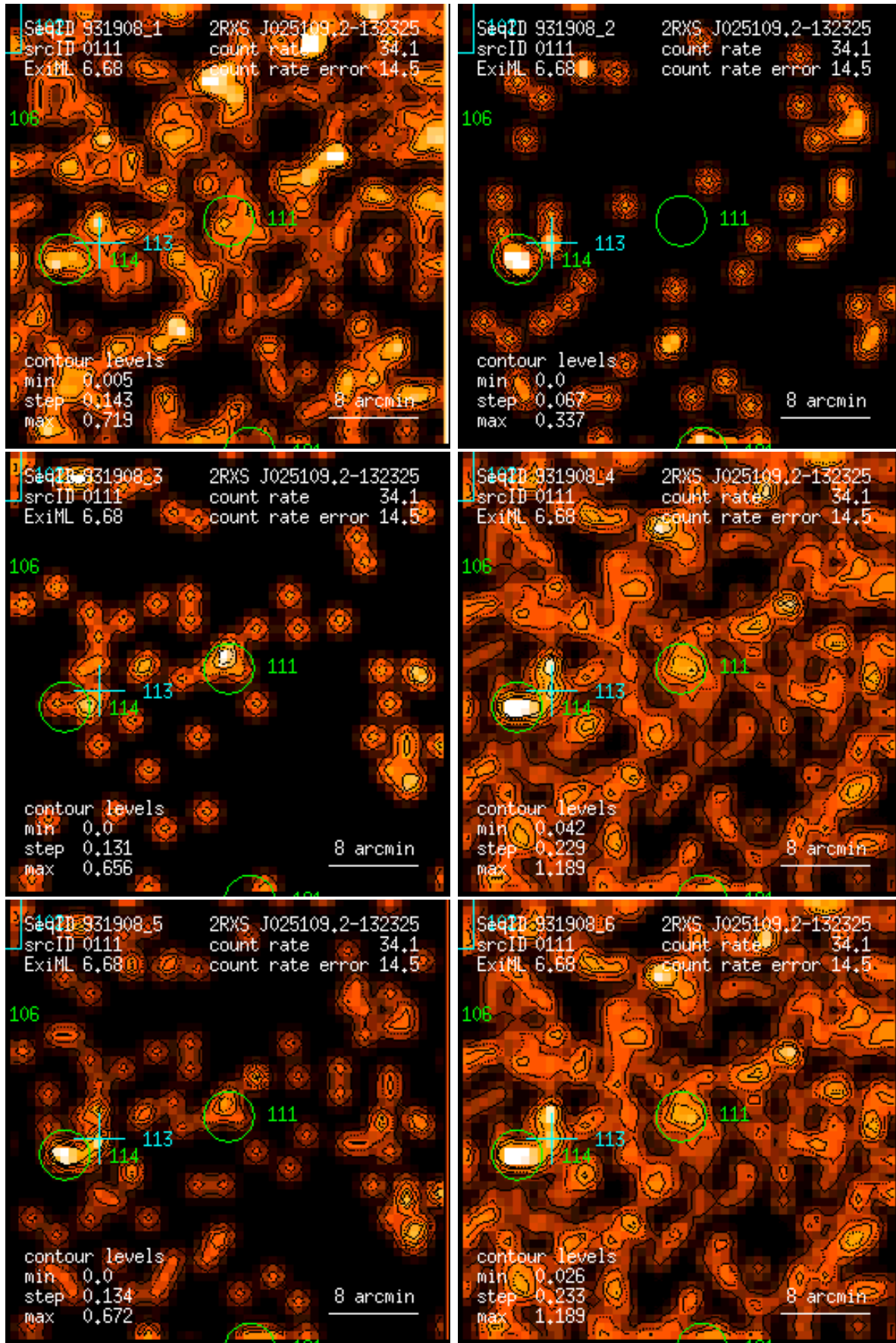
Figure 111: RASS 931908: detection 0111: band rate images, Gaussian filter: (1) PSPC channels 11 – 41, (2) 52 – 90, (3) 91 – 201, (4) 11 – 235, (5) 52 – 201, (6) 11 – 201. Broad band rates in counts/ks. Band rate contour levels in counts/ks/arcmin 2 .
