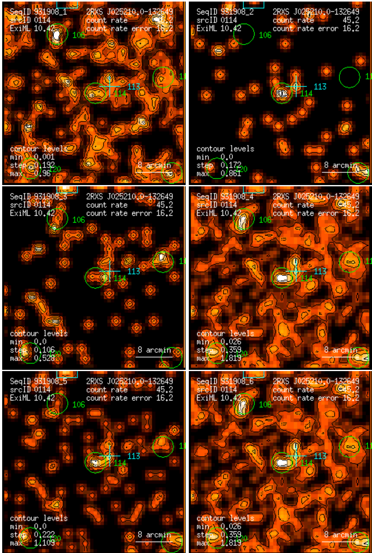
Figure 114: RASS 931908: detection 0114: band rate images, Gaussian filter: (1) PSPC channels 11 – 41, (2) 52 – 90, (3) 91 – 201, (4) 11 – 235, (5) 52 – 201, (6) 11 – 201. Broad band rates in counts/ks. Band rate contour levels in counts/ks/arcmin 2 .
