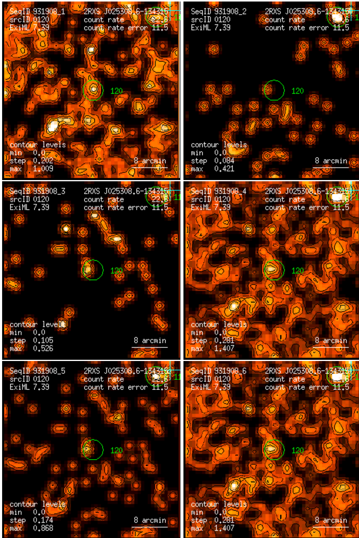
Figure 120: RASS 931908: detection 0120: band rate images, Gaussian filter: (1) PSPC channels 11 – 41, (2) 52 – 90, (3) 91 – 201, (4) 11 – 235, (5) 52 – 201, (6) 11 – 201. Broad band rates in counts/ks. Band rate contour levels in counts/ks/arcmin 2 .
