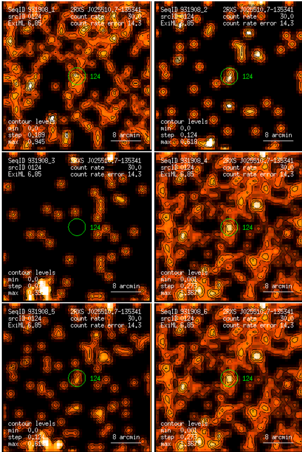
Figure 124: RASS 931908: detection 0124: band rate images, Gaussian filter: (1) PSPC channels 11 – 41, (2) 52 – 90, (3) 91 – 201, (4) 11 – 235, (5) 52 – 201, (6) 11 – 201. Broad band rates in counts/ks. Band rate contour levels in counts/ks/arcmin 2 .
