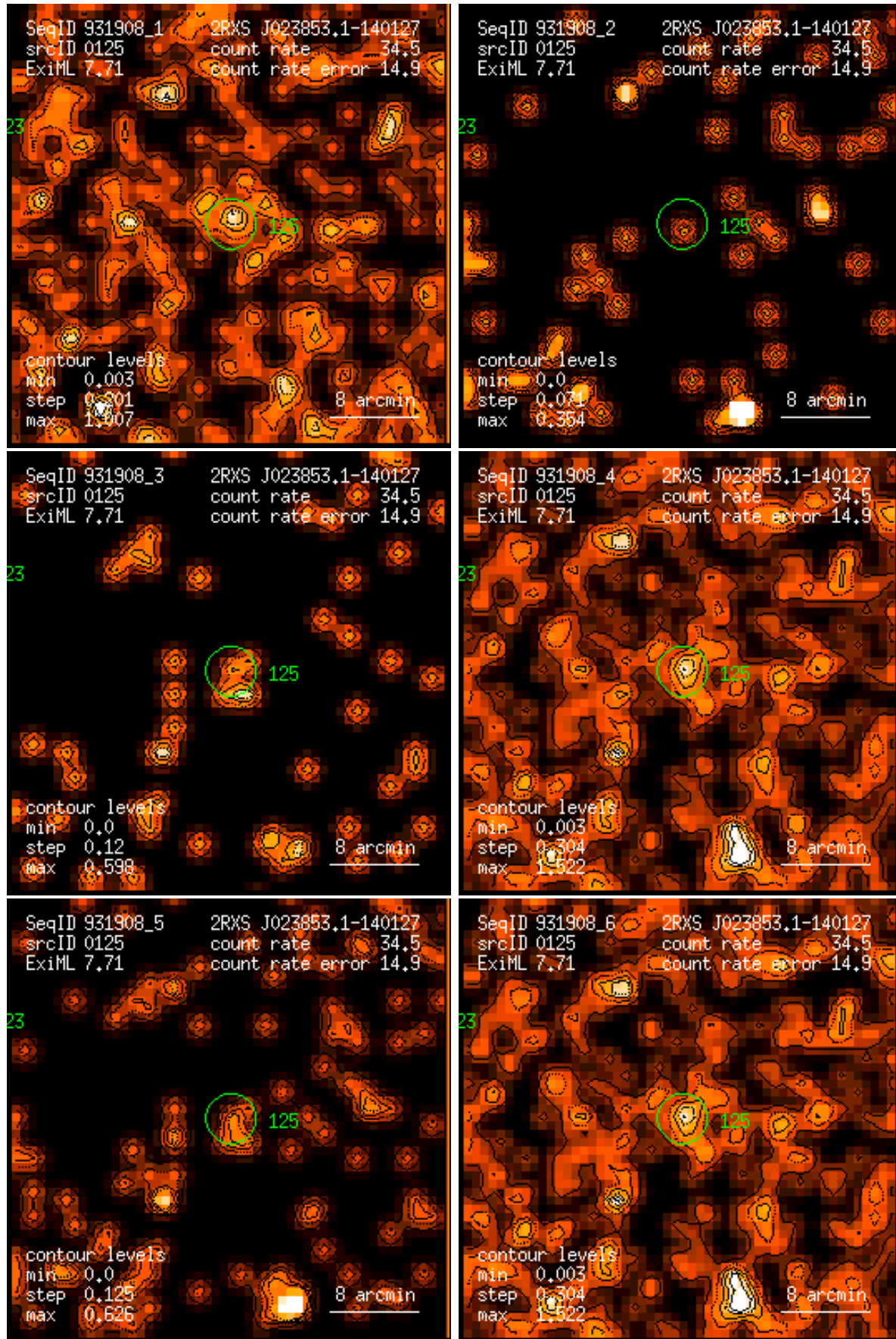
Figure 125: RASS 931908: detection 0125: band rate images, Gaussian filter: (1) PSPC channels 11 – 41, (2) 52 – 90, (3) 91 – 201, (4) 11 – 235, (5) 52 – 201, (6) 11 – 201. Broad band rates in counts/ks. Band rate contour levels in counts/ks/arcmin 2 .
