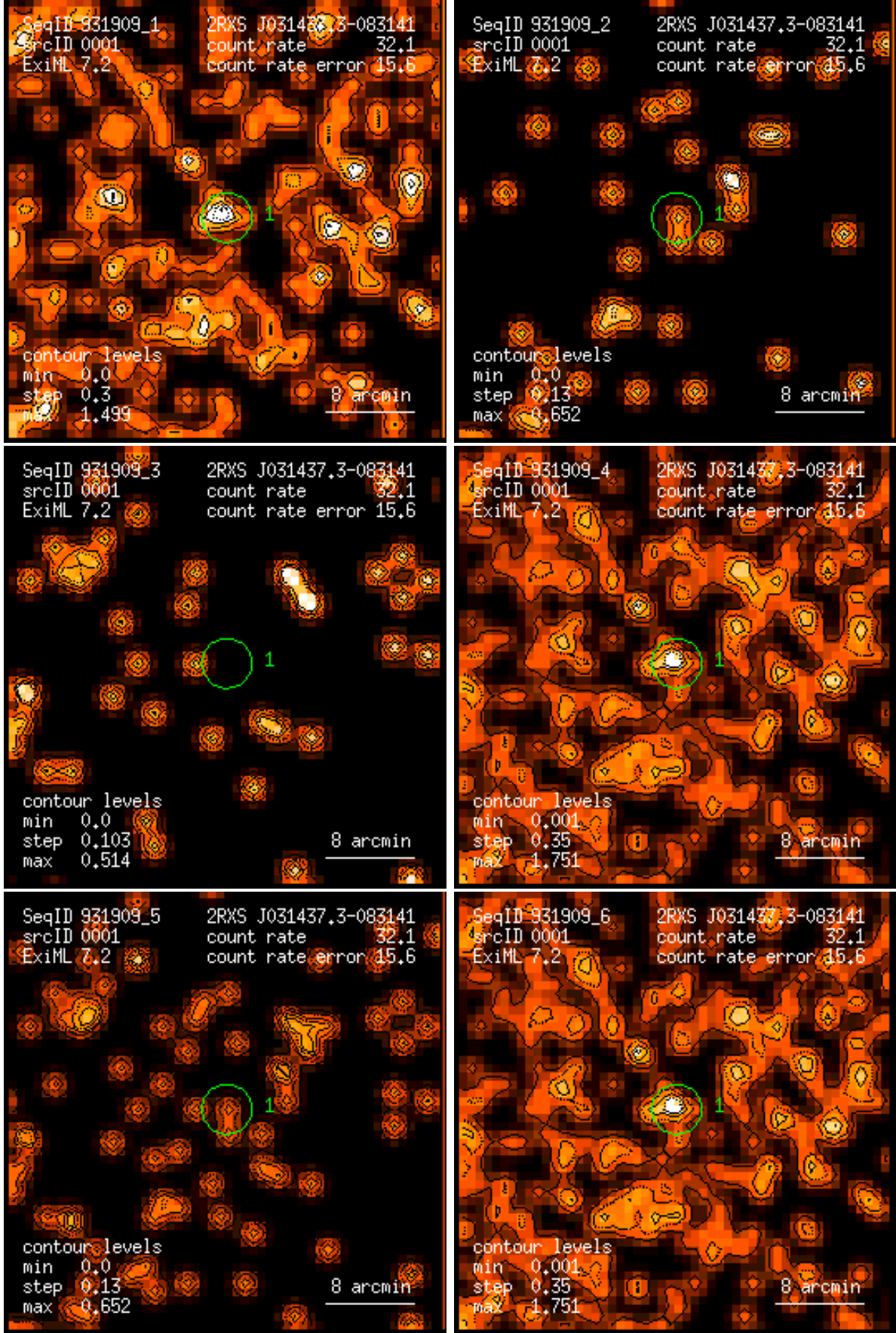
Figure 1: RASS 931909: detection 0001: band rate images, Gaussian filter: (1) PSPC channels 11 – 41, (2) 52 – 90, (3) 91 – 201, (4) 11 – 235, (5) 52 – 201, (6) 11 – 201. Broad band rates in counts/ks. Band rate contour levels in counts/ks/arcmin 2 .
