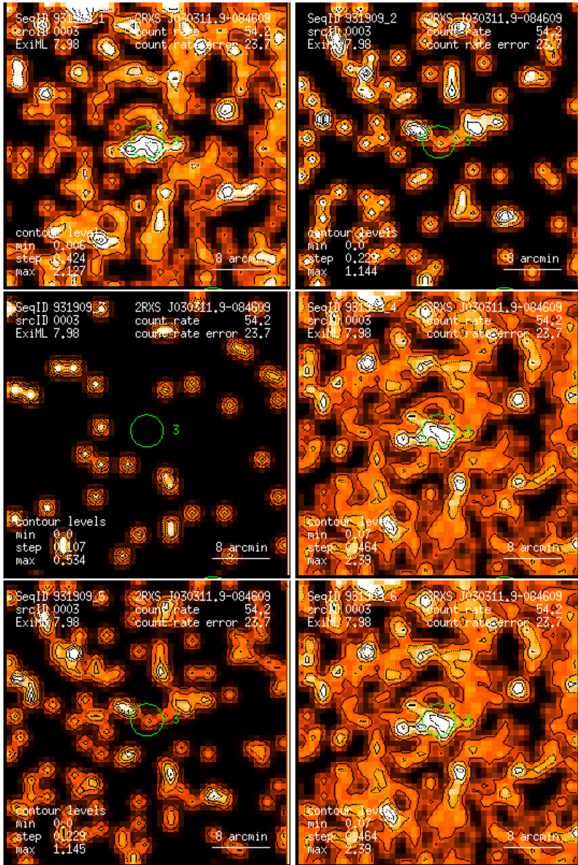
Figure 3: RASS 931909: detection 0003: band rate images, Gaussian filter: (1) PSPC channels 11 – 41, (2) 52 – 90, (3) 91 – 201, (4) 11 – 235, (5) 52 – 201, (6) 11 – 201. Broad band rates in counts/ks. Band rate contour levels in counts/ks/arcmin 2 .
