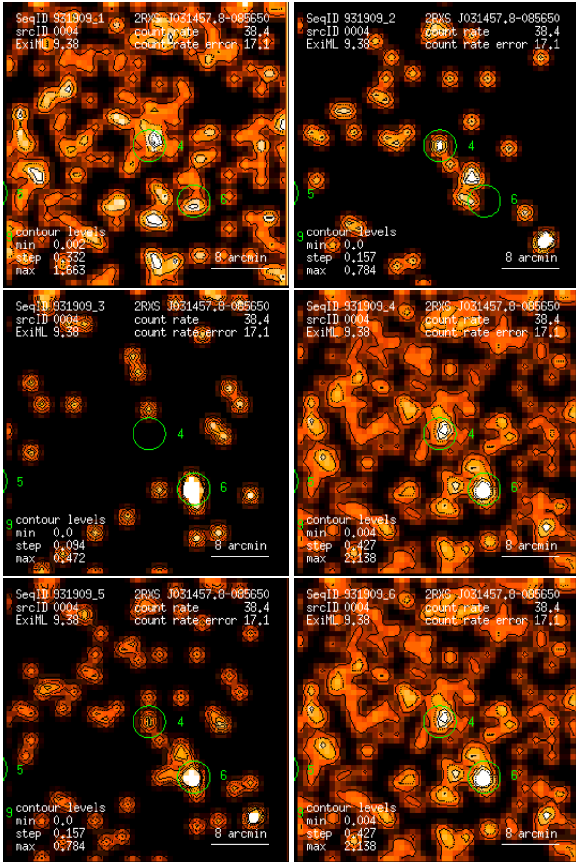
Figure 4: RASS 931909: detection 0004: band rate images, Gaussian filter: (1) PSPC channels 11 – 41, (2) 52 – 90, (3) 91 – 201, (4) 11 – 235, (5) 52 – 201, (6) 11 – 201. Broad band rates in counts/ks. Band rate contour levels in counts/ks/arcmin 2 .
