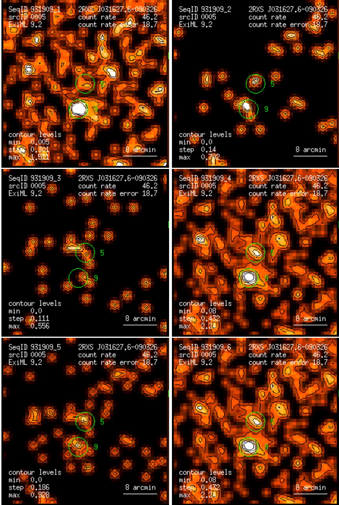
Figure 5: RASS 931909: detection 0005: band rate images, Gaussian filter: (1) PSPC channels 11 – 41, (2) 52 – 90, (3) 91 – 201, (4) 11 – 235, (5) 52 – 201, (6) 11 – 201. Broad band rates in counts/ks. Band rate contour levels in counts/ks/arcmin 2 .
