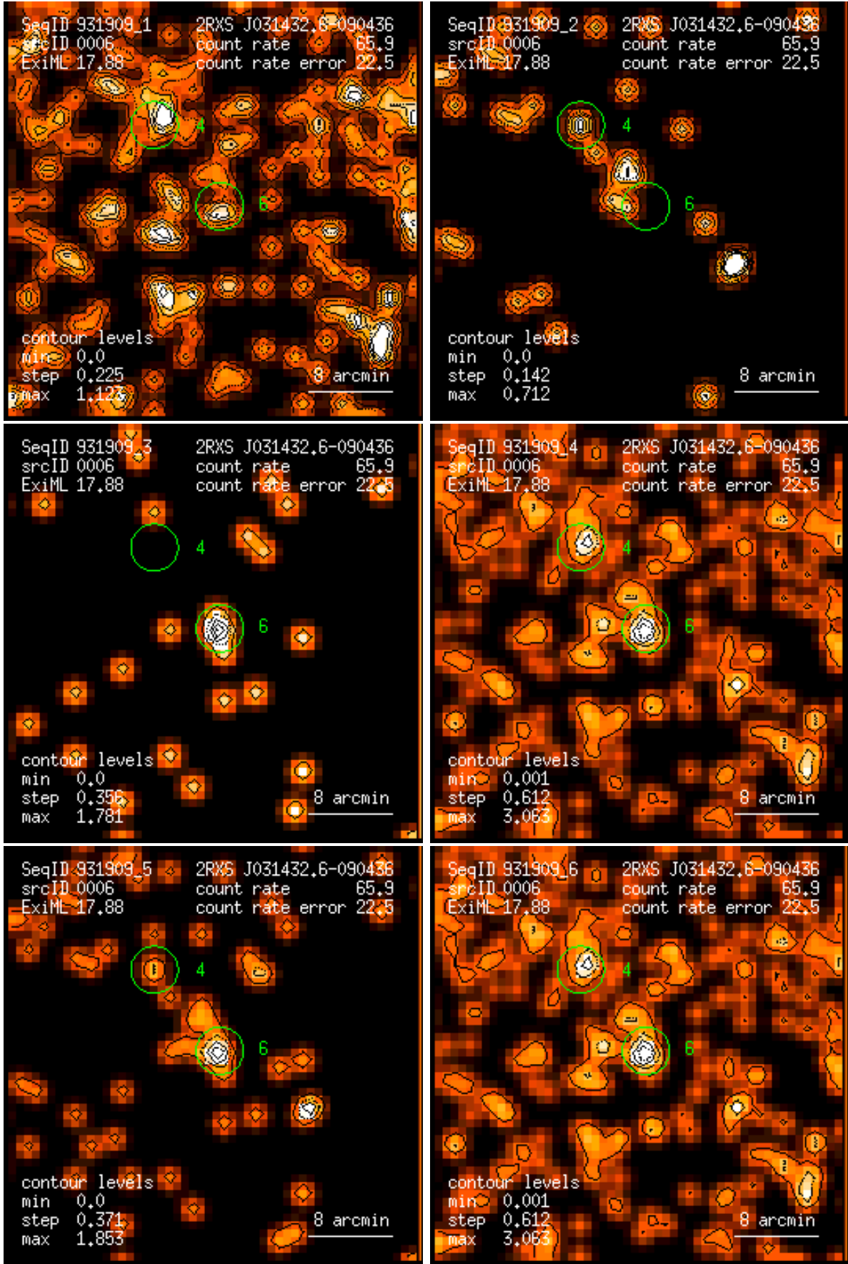
Figure 6: RASS 931909: detection 0006: band rate images, Gaussian filter: (1) PSPC channels 11 – 41, (2) 52 – 90, (3) 91 – 201, (4) 11 – 235, (5) 52 – 201, (6) 11 – 201. Broad band rates in counts/ks. Band rate contour levels in counts/ks/arcmin 2 .
