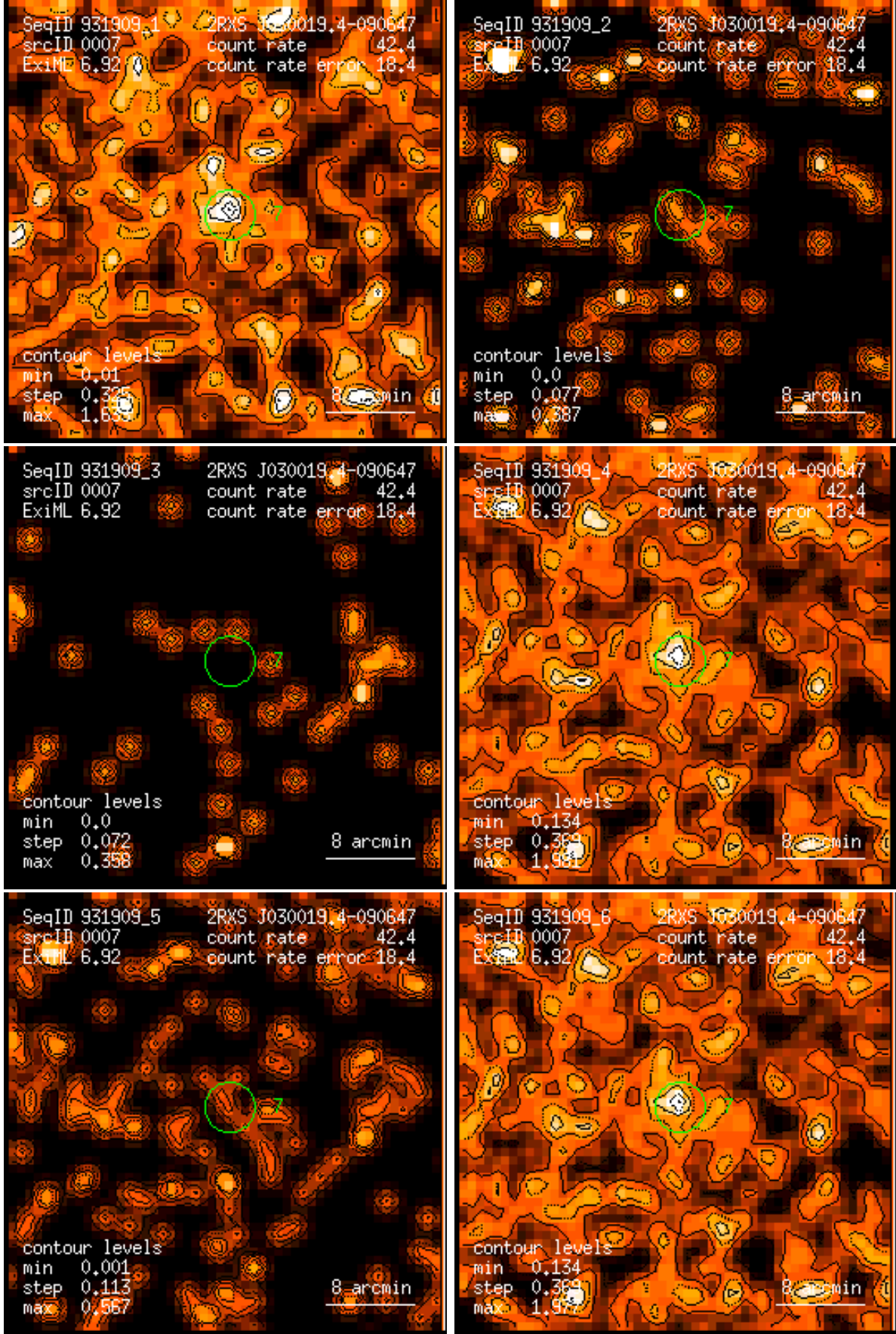
Figure 7: RASS 931909: detection 0007: band rate images, Gaussian filter: (1) PSPC channels 11 – 41, (2) 52 – 90, (3) 91 – 201, (4) 11 – 235, (5) 52 – 201, (6) 11 – 201. Broad band rates in counts/ks. Band rate contour levels in counts/ks/arcmin 2 .
