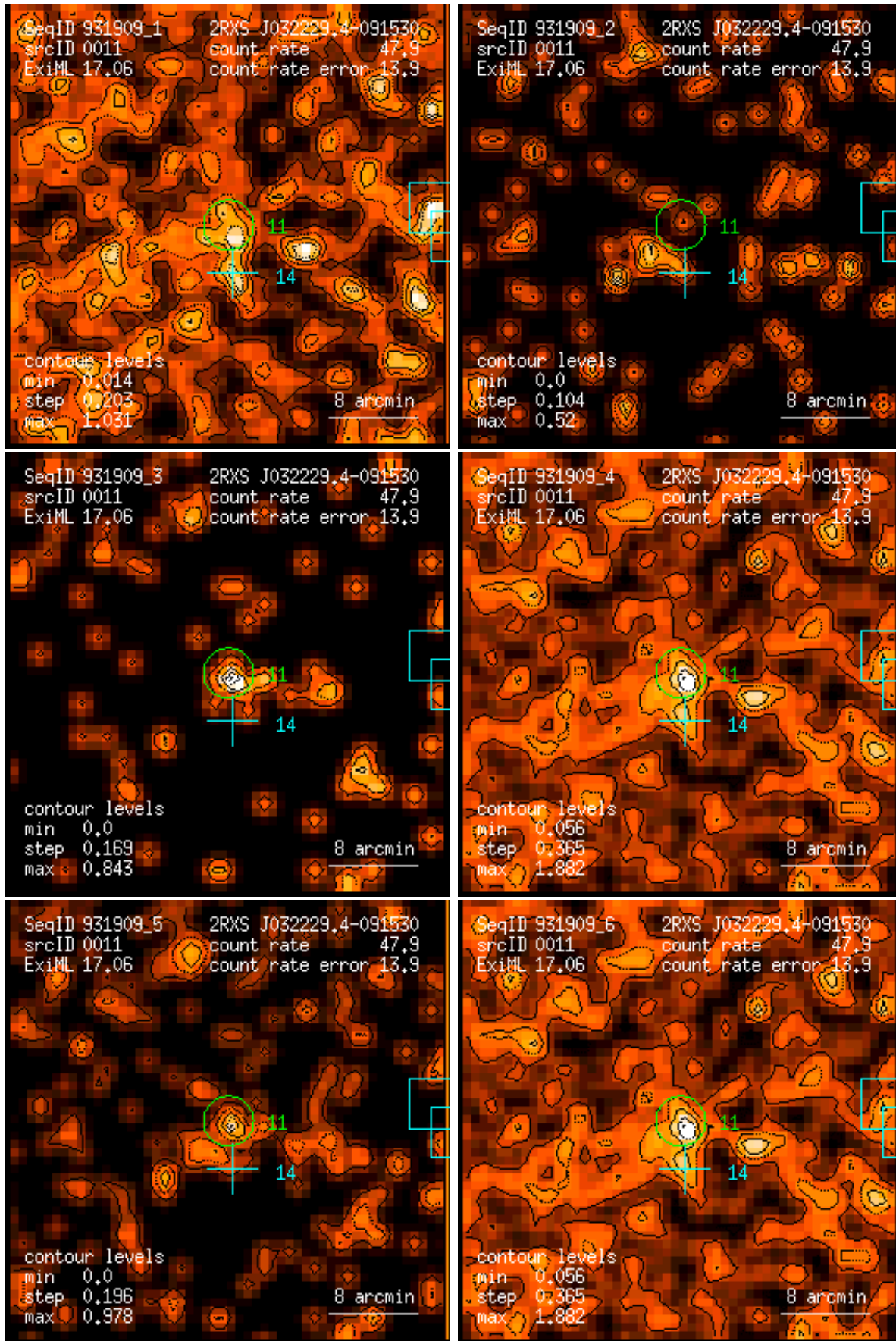
Figure 11: RASS 931909: detection 0011: band rate images, Gaussian filter: (1) PSPC channels 11 – 41, (2) 52 – 90, (3) 91 – 201, (4) 11 – 235, (5) 52 – 201, (6) 11 – 201. Broad band rates in counts/ks. Band rate contour levels in counts/ks/arcmin 2 .
