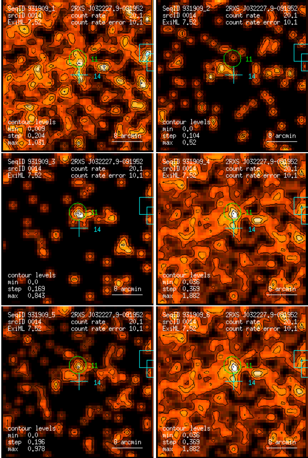
Figure 14: RASS 931909: detection 0014: band rate images, Gaussian filter: (1) PSPC channels 11 – 41, (2) 52 – 90, (3) 91 – 201, (4) 11 – 235, (5) 52 – 201, (6) 11 – 201. Broad band rates in counts/ks. Band rate contour levels in counts/ks/arcmin 2 .
