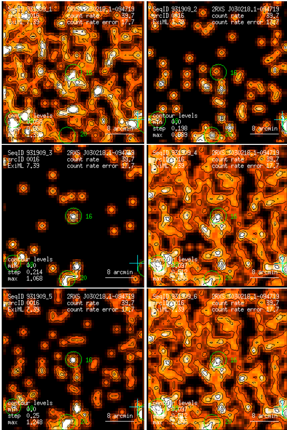
Figure 16: RASS 931909: detection 0016: band rate images, Gaussian filter: (1) PSPC channels 11 – 41, (2) 52 – 90, (3) 91 – 201, (4) 11 – 235, (5) 52 – 201, (6) 11 – 201. Broad band rates in counts/ks. Band rate contour levels in counts/ks/arcmin 2 .
