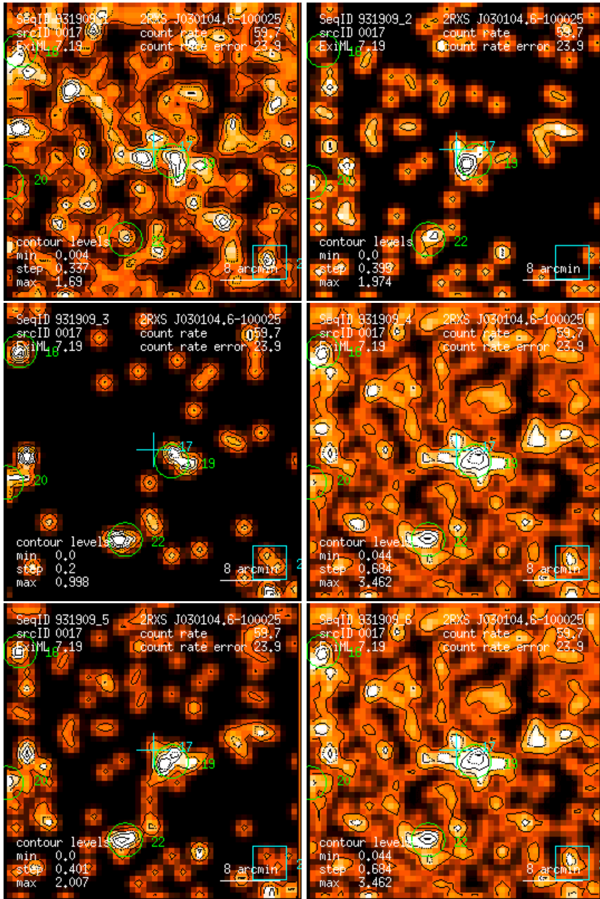
Figure 17: RASS 931909: detection 0017: band rate images, Gaussian filter: (1) PSPC channels 11 – 41, (2) 52 – 90, (3) 91 – 201, (4) 11 – 235, (5) 52 – 201, (6) 11 – 201. Broad band rates in counts/ks. Band rate contour levels in counts/ks/arcmin 2 .
