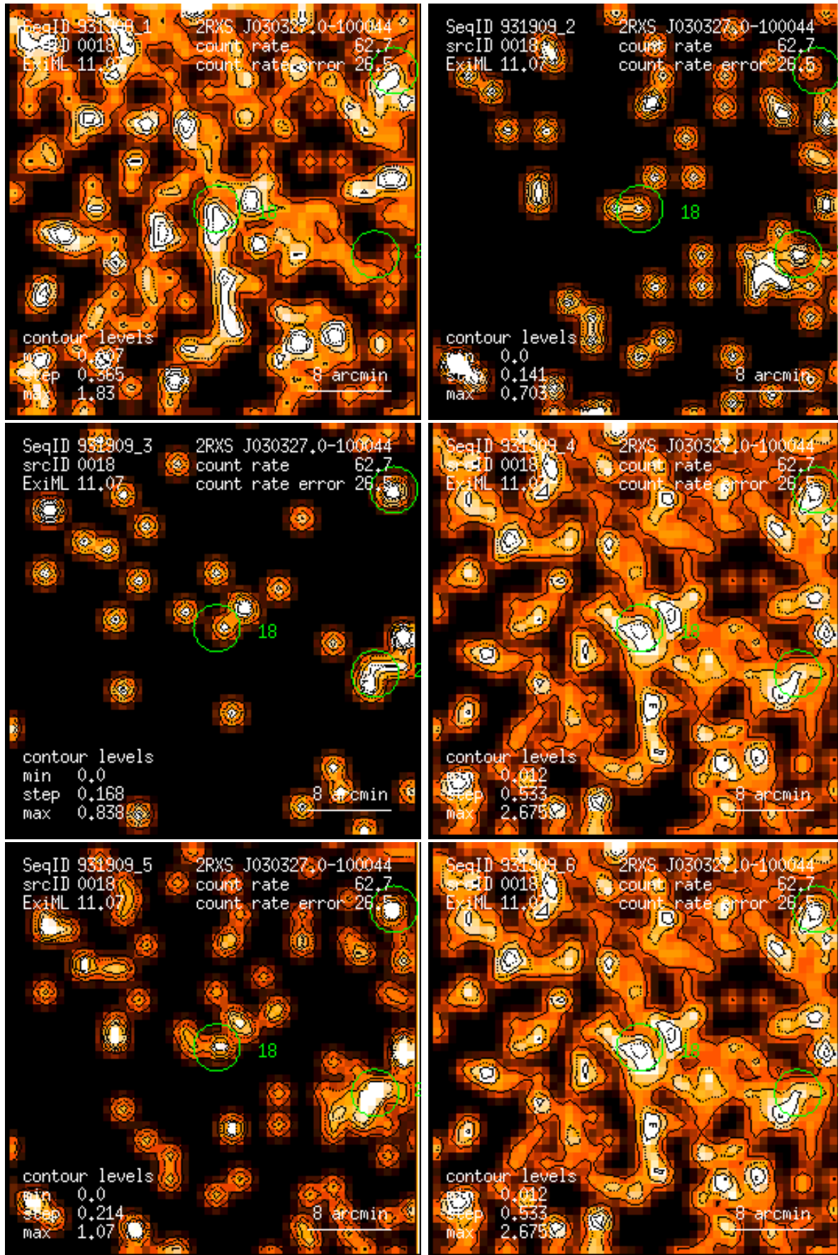
Figure 18: RASS 931909: detection 0018: band rate images, Gaussian filter: (1) PSPC channels 11 – 41, (2) 52 – 90, (3) 91 – 201, (4) 11 – 235, (5) 52 – 201, (6) 11 – 201. Broad band rates in counts/ks. Band rate contour levels in counts/ks/arcmin 2 .
