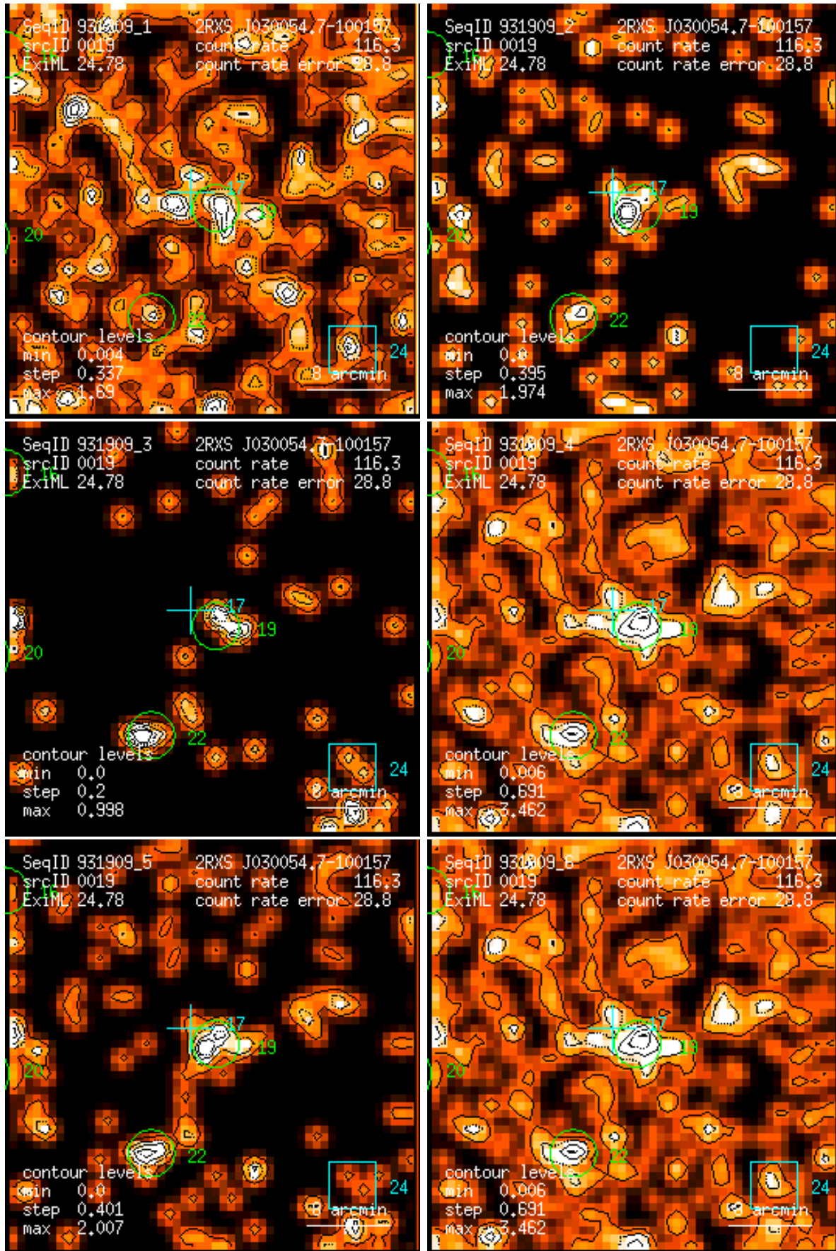
Figure 19: RASS 931909: detection 0019: band rate images, Gaussian filter: (1) PSPC channels 11 – 41, (2) 52 – 90, (3) 91 – 201, (4) 11 – 235, (5) 52 – 201, (6) 11 – 201. Broad band rates in counts/ks. Band rate contour levels in counts/ks/arcmin 2 .
