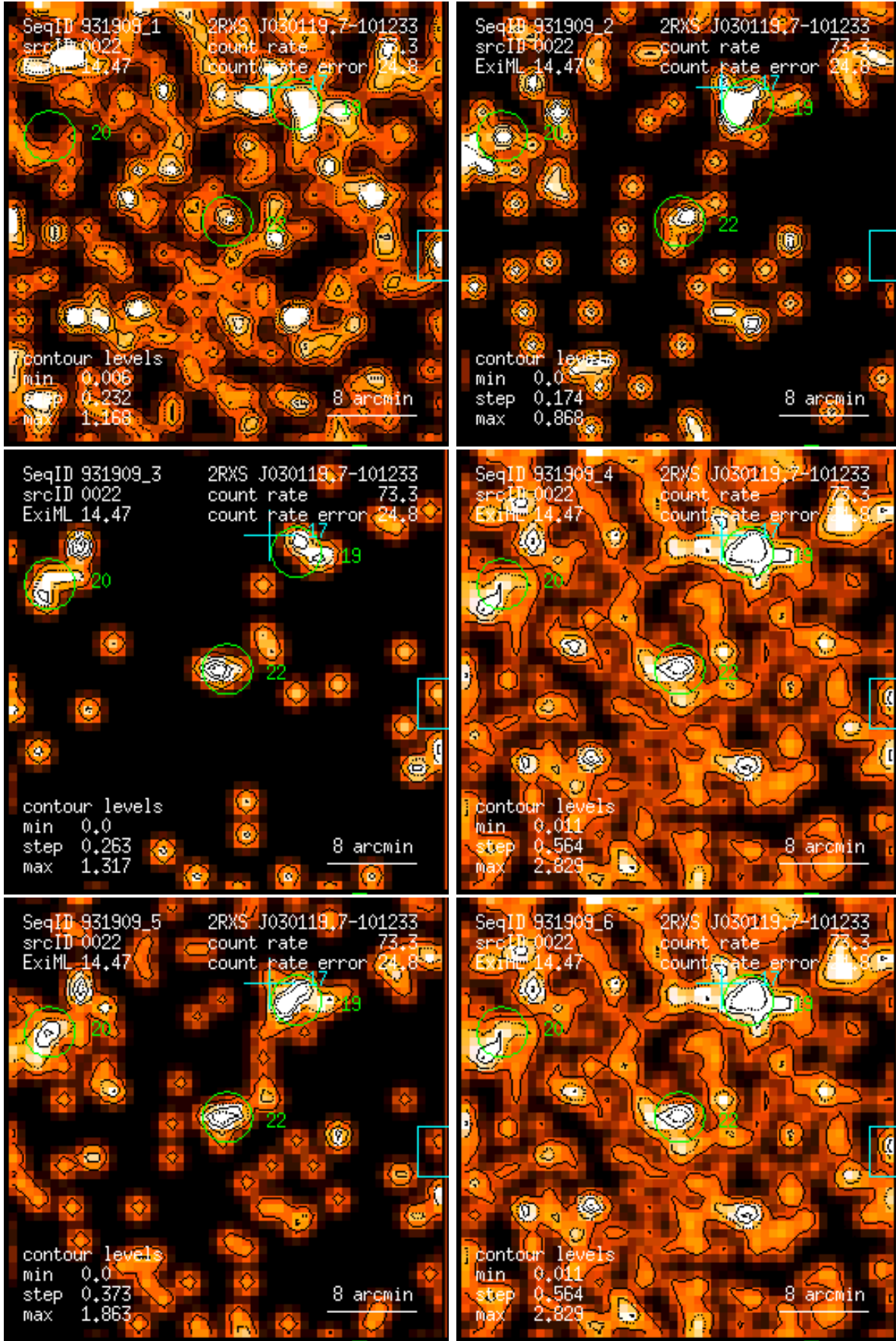
Figure 22: RASS 931909: detection 0022: band rate images, Gaussian filter: (1) PSPC channels 11 – 41, (2) 52 – 90, (3) 91 – 201, (4) 11 – 235, (5) 52 – 201, (6) 11 – 201. Broad band rates in counts/ks. Band rate contour levels in counts/ks/arcmin 2 .
