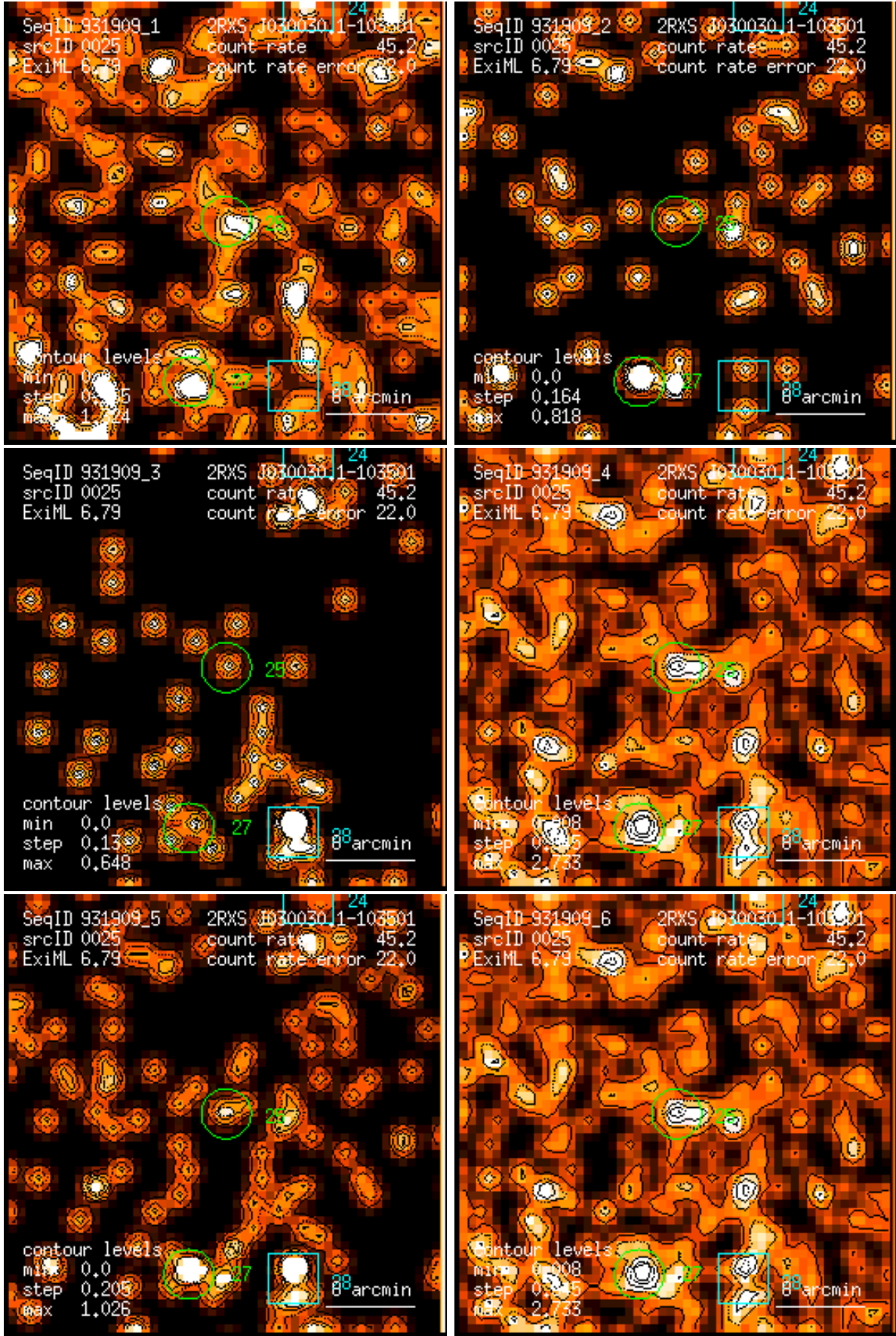
Figure 25: RASS 931909: detection 0025: band rate images, Gaussian filter: (1) PSPC channels 11 – 41, (2) 52 – 90, (3) 91 – 201, (4) 11 – 235, (5) 52 – 201, (6) 11 – 201. Broad band rates in counts/ks. Band rate contour levels in counts/ks/arcmin 2 .
