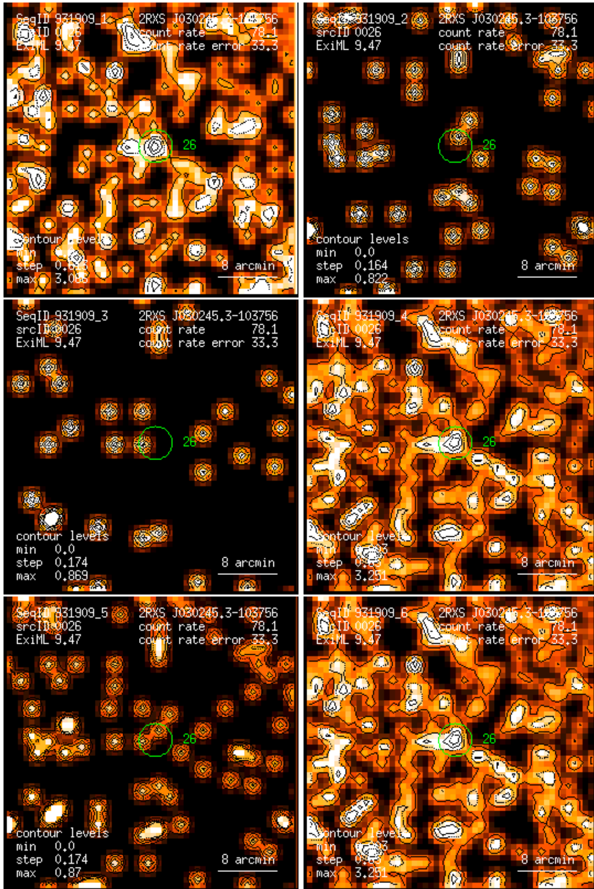
Figure 26: RASS 931909: detection 0026: band rate images, Gaussian filter: (1) PSPC channels 11 – 41, (2) 52 – 90, (3) 91 – 201, (4) 11 – 235, (5) 52 – 201, (6) 11 – 201. Broad band rates in counts/ks. Band rate contour levels in counts/ks/arcmin 2 .
