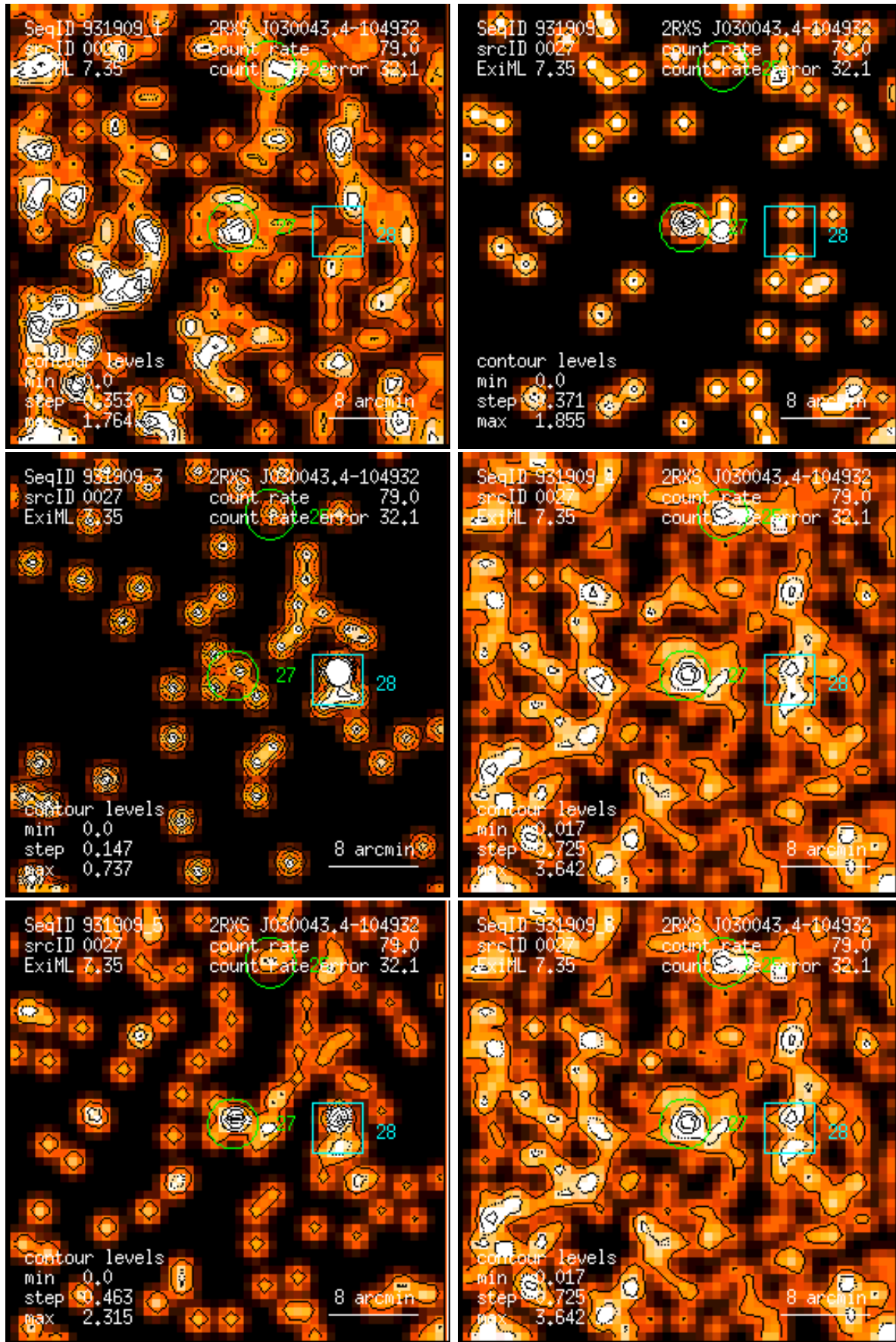
Figure 27: RASS 931909: detection 0027: band rate images, Gaussian filter: (1) PSPC channels 11 – 41, (2) 52 – 90, (3) 91 – 201, (4) 11 – 235, (5) 52 – 201, (6) 11 – 201. Broad band rates in counts/ks. Band rate contour levels in counts/ks/arcmin 2 .
