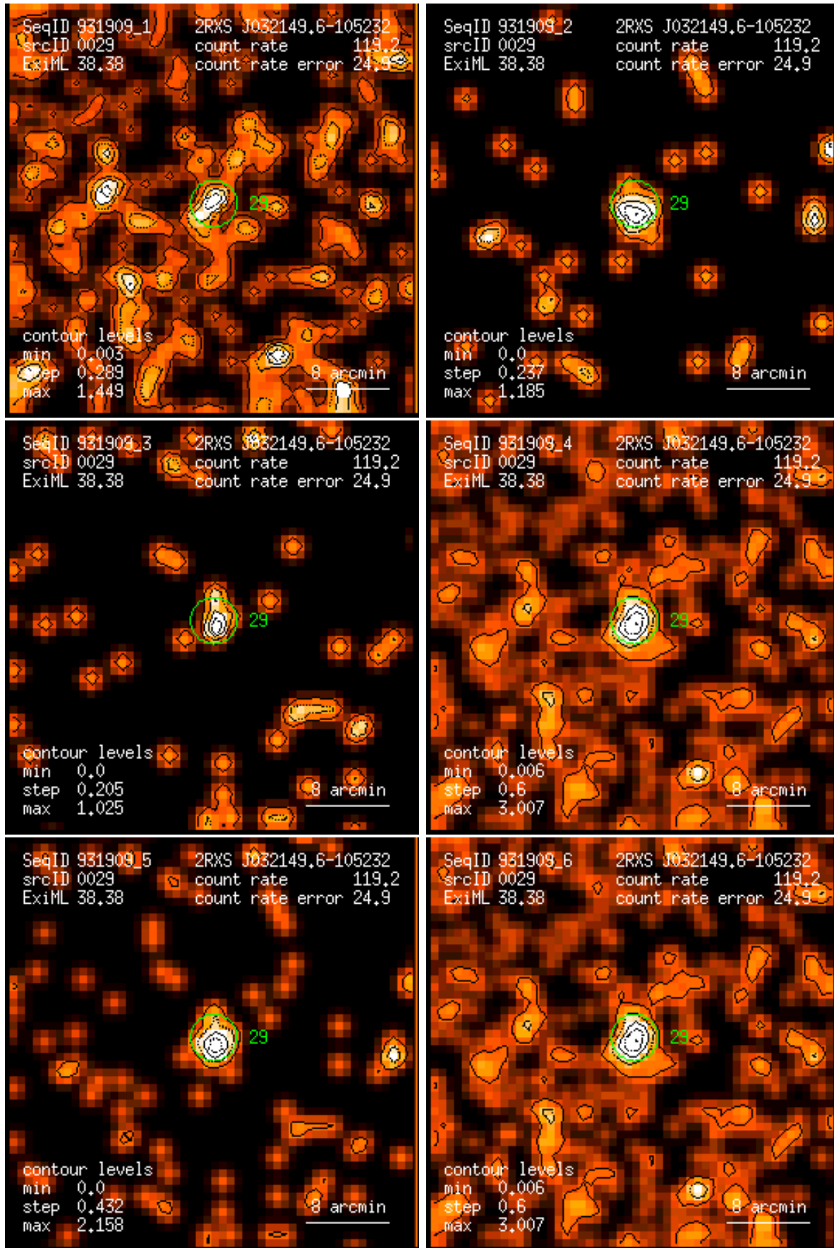
Figure 29: RASS 931909: detection 0029: band rate images, Gaussian filter: (1) PSPC channels 11 – 41, (2) 52 – 90, (3) 91 – 201, (4) 11 – 235, (5) 52 – 201, (6) 11 – 201. Broad band rates in counts/ks. Band rate contour levels in counts/ks/arcmin 2 .
