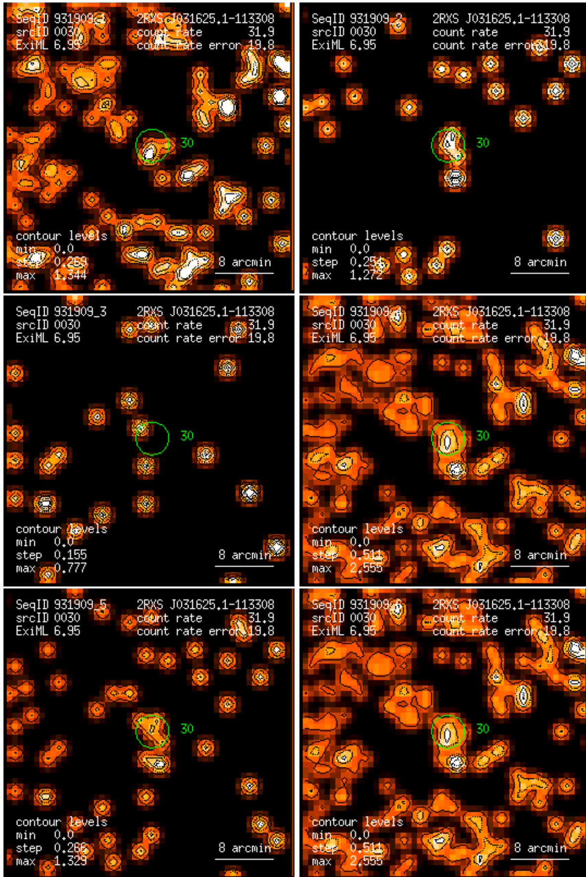
Figure 30: RASS 931909: detection 0030: band rate images, Gaussian filter: (1) PSPC channels 11 – 41, (2) 52 – 90, (3) 91 – 201, (4) 11 – 235, (5) 52 – 201, (6) 11 – 201. Broad band rates in counts/ks. Band rate contour levels in counts/ks/arcmin 2 .
