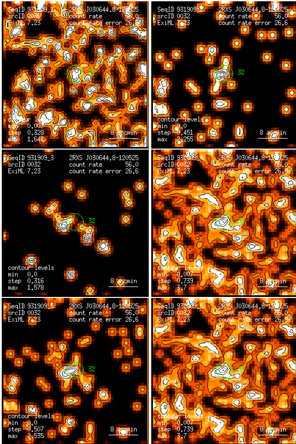
Figure 32: RASS 931909: detection 0032: band rate images, Gaussian filter: (1) PSPC channels 11 – 41, (2) 52 – 90, (3) 91 – 201, (4) 11 – 235, (5) 52 – 201, (6) 11 – 201. Broad band rates in counts/ks. Band rate contour levels in counts/ks/arcmin 2 .
