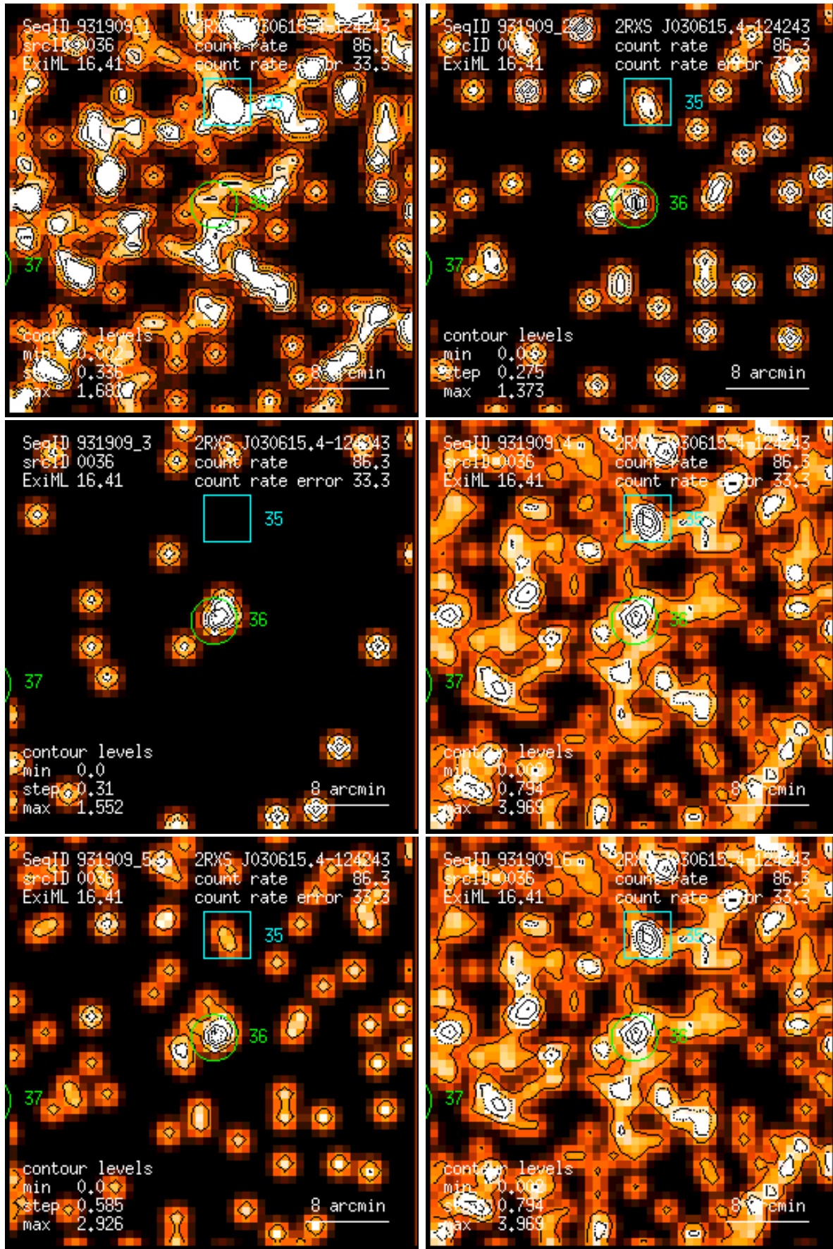
Figure 36: RASS 931909: detection 0036: band rate images, Gaussian filter: (1) PSPC channels 11 – 41, (2) 52 – 90, (3) 91 – 201, (4) 11 – 235, (5) 52 – 201, (6) 11 – 201. Broad band rates in counts/ks. Band rate contour levels in counts/ks/arcmin 2 .
