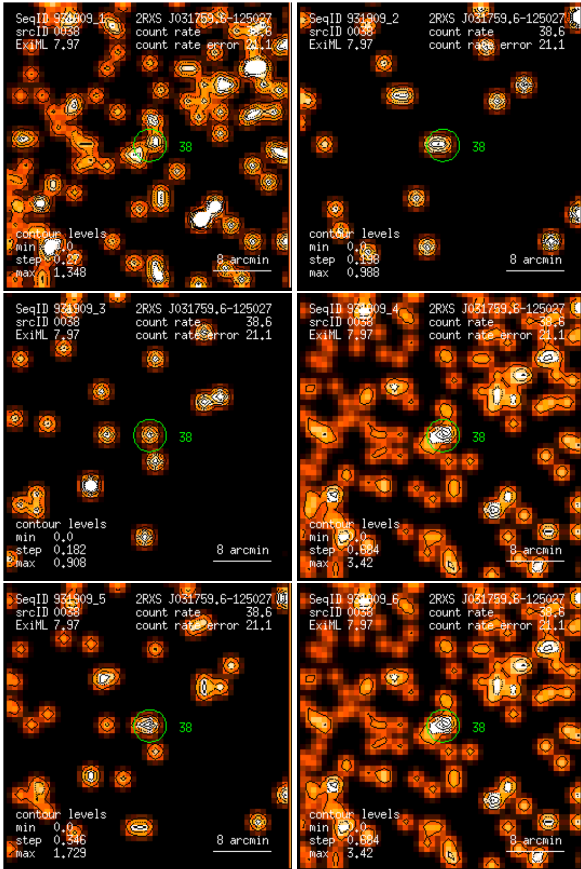
Figure 38: RASS 931909: detection 0038: band rate images, Gaussian filter: (1) PSPC channels 11 – 41, (2) 52 – 90, (3) 91 – 201, (4) 11 – 235, (5) 52 – 201, (6) 11 – 201. Broad band rates in counts/ks. Band rate contour levels in counts/ks/arcmin 2 .
