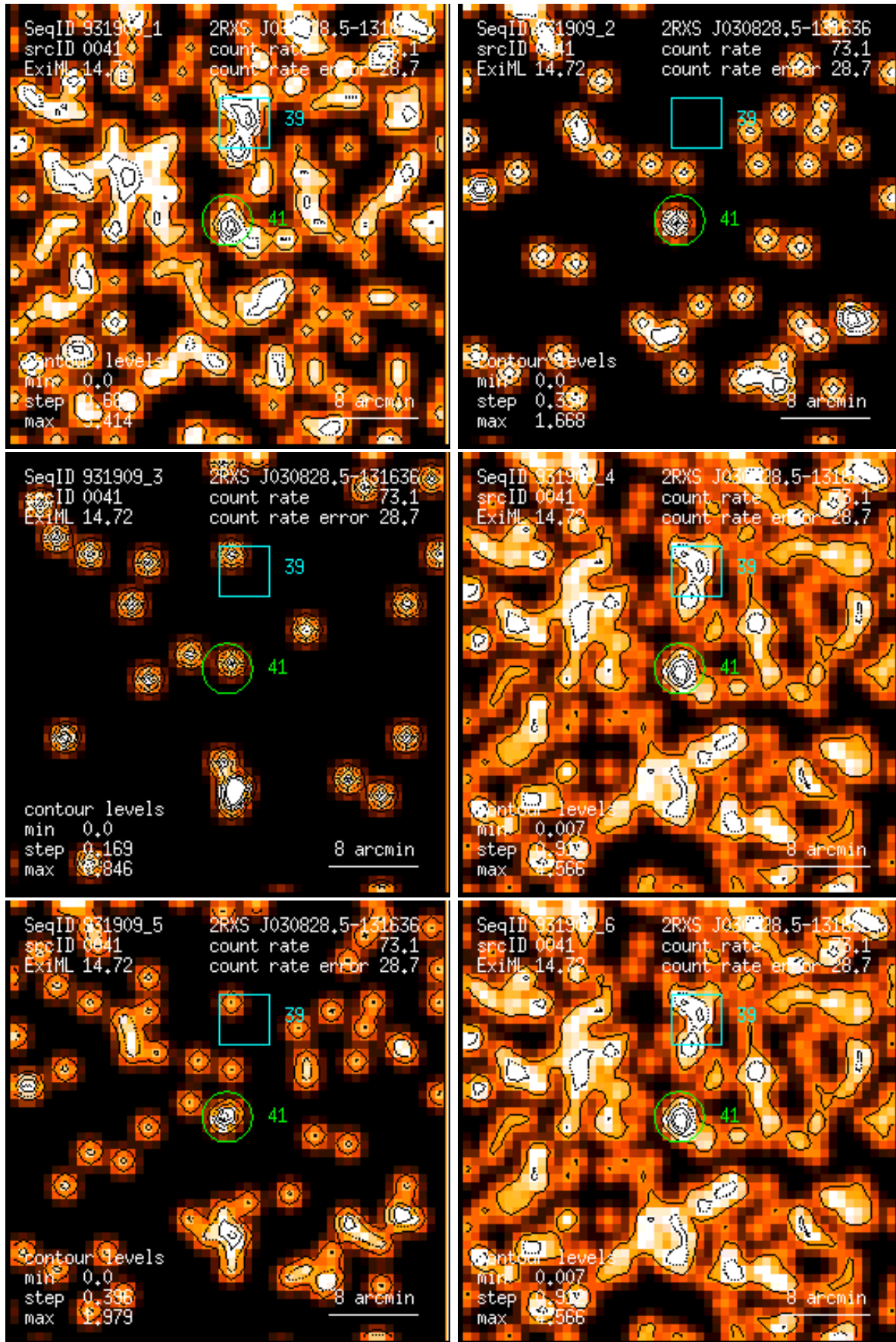
Figure 41: RASS 931909: detection 0041: band rate images, Gaussian filter: (1) PSPC channels 11 – 41, (2) 52 – 90, (3) 91 – 201, (4) 11 – 235, (5) 52 – 201, (6) 11 – 201. Broad band rates in counts/ks. Band rate contour levels in counts/ks/arcmin 2 .
