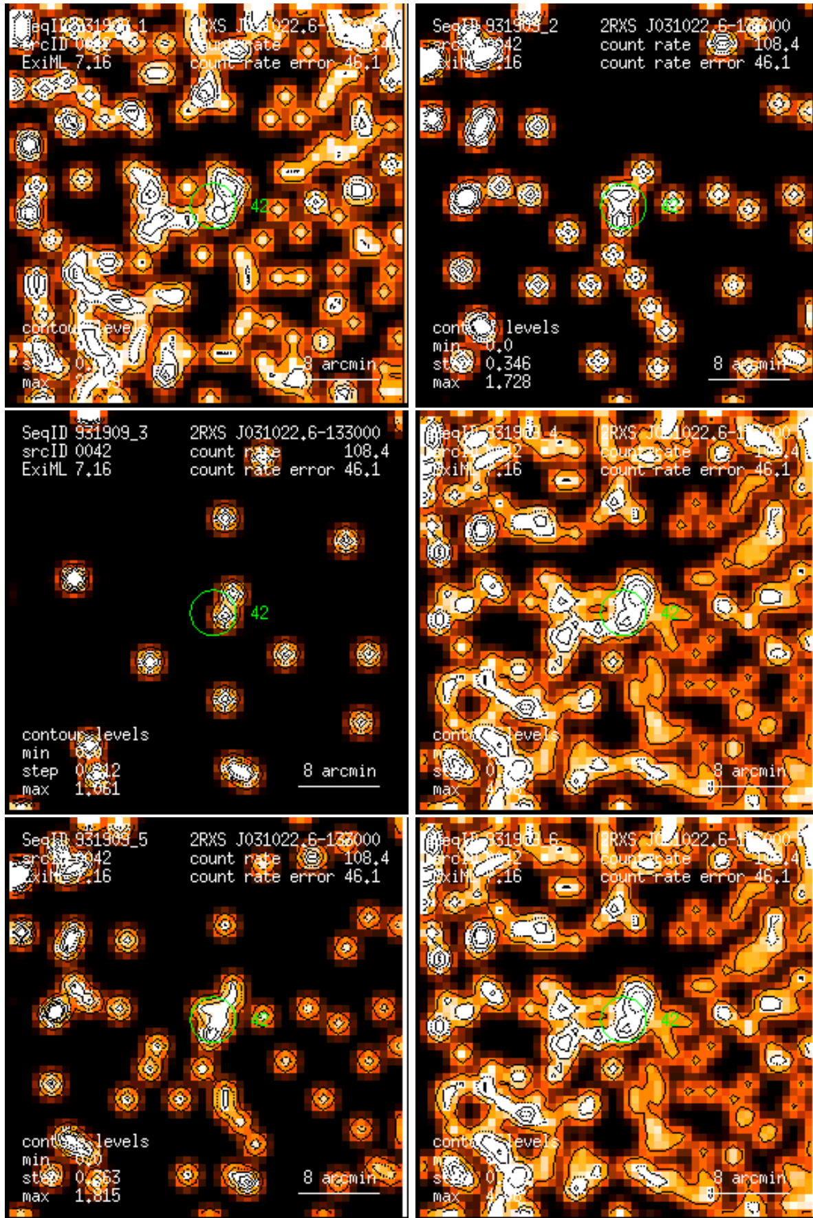
Figure 42: RASS 931909: detection 0042: band rate images, Gaussian filter: (1) PSPC channels 11 – 41, (2) 52 – 90, (3) 91 – 201, (4) 11 – 235, (5) 52 – 201, (6) 11 – 201. Broad band rates in counts/ks. Band rate contour levels in counts/ks/arcmin 2 .
