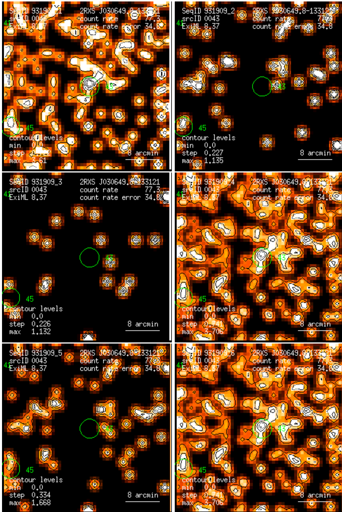
Figure 43: RASS 931909: detection 0043: band rate images, Gaussian filter: (1) PSPC channels 11 – 41, (2) 52 – 90, (3) 91 – 201, (4) 11 – 235, (5) 52 – 201, (6) 11 – 201. Broad band rates in counts/ks. Band rate contour levels in counts/ks/arcmin 2 .
