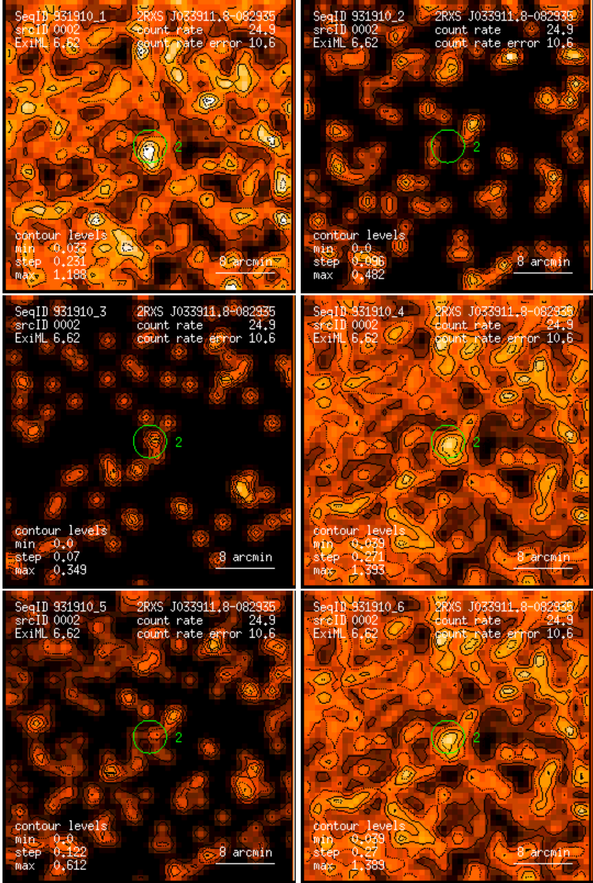
Figure 2: RASS 931910: detection 0002: band rate images, Gaussian filter: (1) PSPC channels 11 – 41, (2) 52 – 90, (3) 91 – 201, (4) 11 – 235, (5) 52 – 201, (6) 11 – 201. Broad band rates in counts/ks. Band rate contour levels in counts/ks/arcmin 2 .
