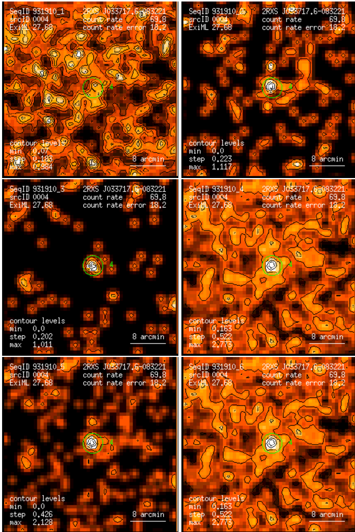
Figure 4: RASS 931910: detection 0004: band rate images, Gaussian filter: (1) PSPC channels 11 – 41, (2) 52 – 90, (3) 91 – 201, (4) 11 – 235, (5) 52 – 201, (6) 11 – 201. Broad band rates in counts/ks. Band rate contour levels in counts/ks/arcmin 2 .
