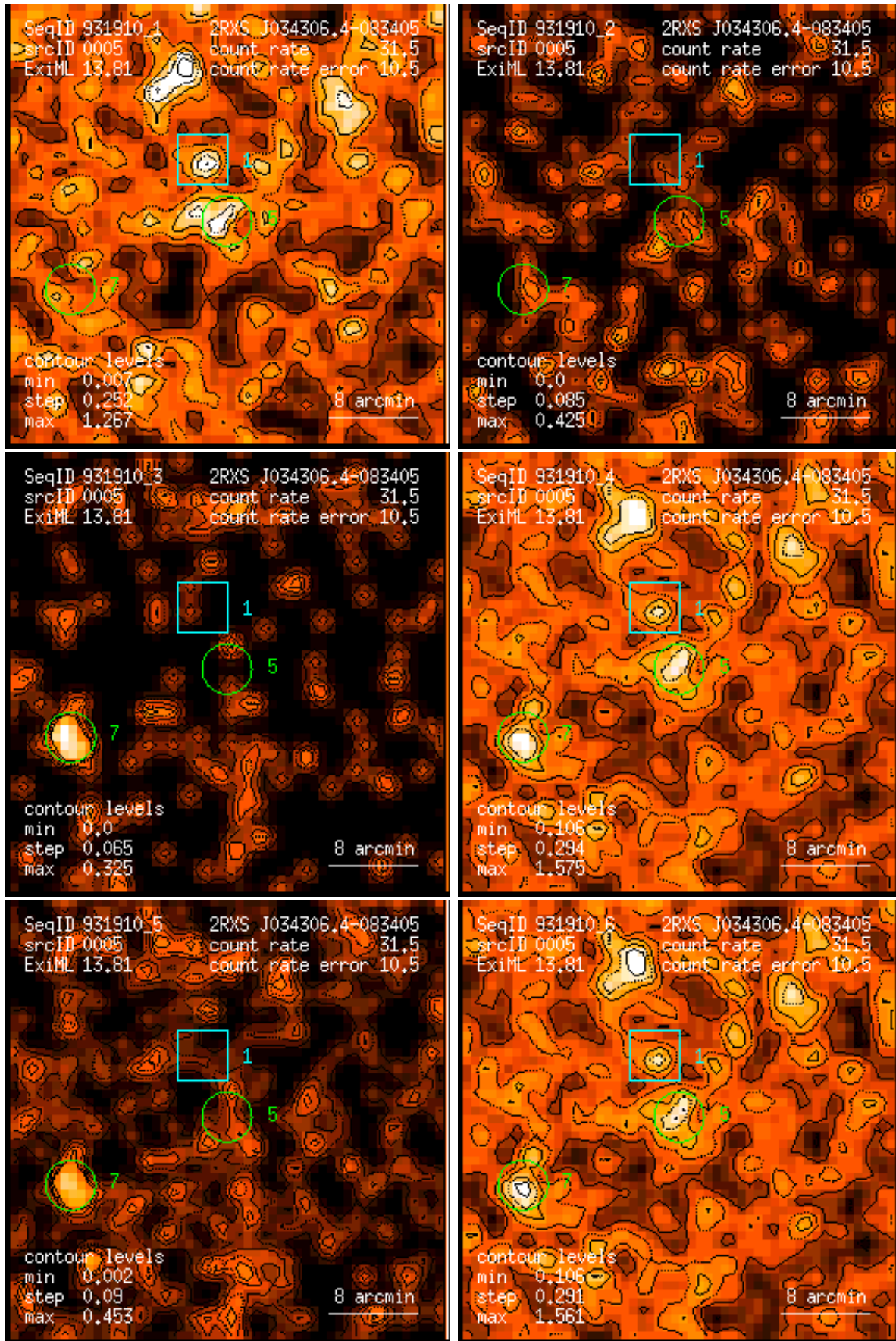
Figure 5: RASS 931910: detection 0005: band rate images, Gaussian filter: (1) PSPC channels 11 – 41, (2) 52 – 90, (3) 91 – 201, (4) 11 – 235, (5) 52 – 201, (6) 11 – 201. Broad band rates in counts/ks. Band rate contour levels in counts/ks/arcmin 2 .
