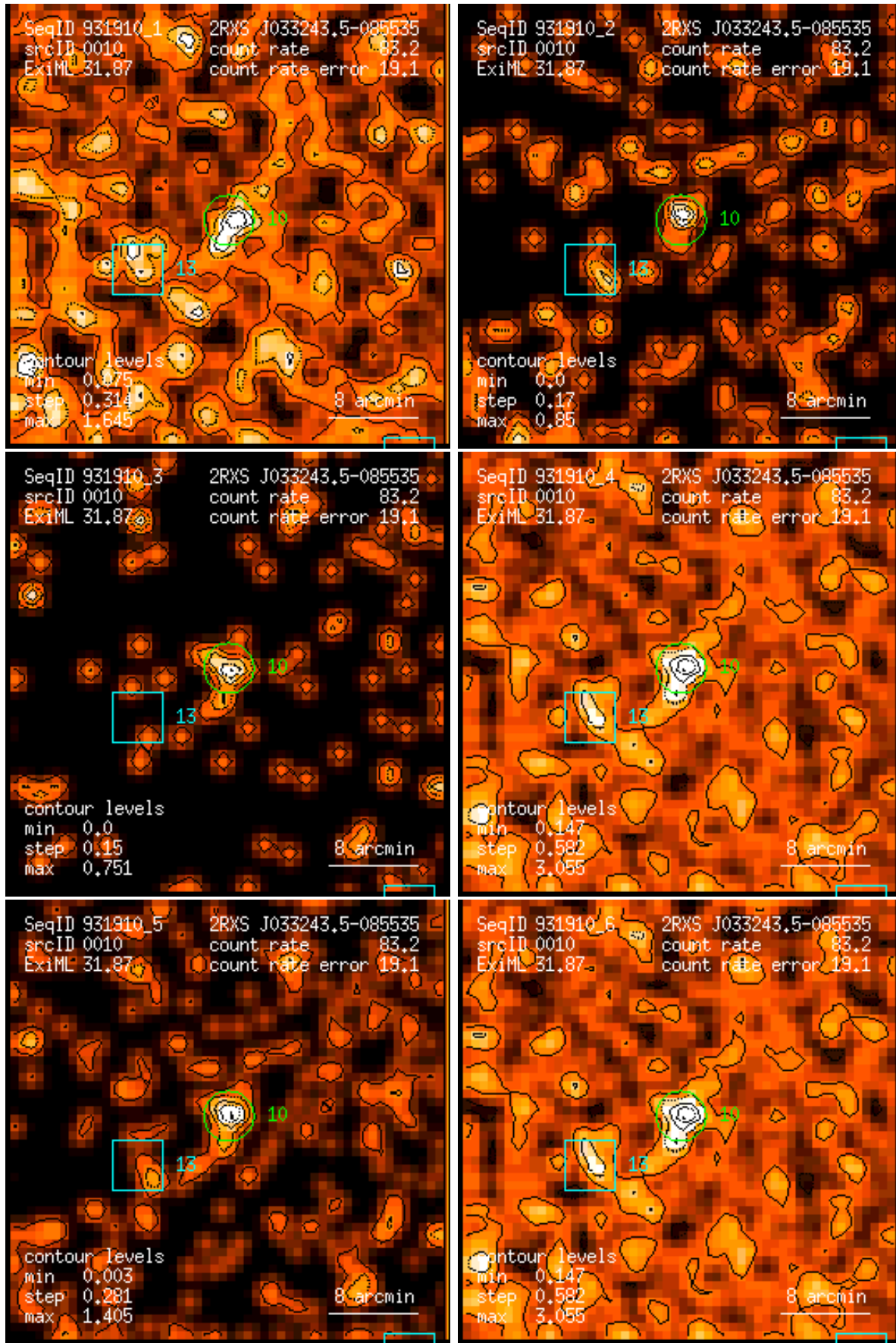
Figure 10: RASS 931910: detection 0010: band rate images, Gaussian filter: (1) PSPC channels 11 – 41, (2) 52 – 90, (3) 91 – 201, (4) 11 – 235, (5) 52 – 201, (6) 11 – 201. Broad band rates in counts/ks. Band rate contour levels in counts/ks/arcmin 2 .
