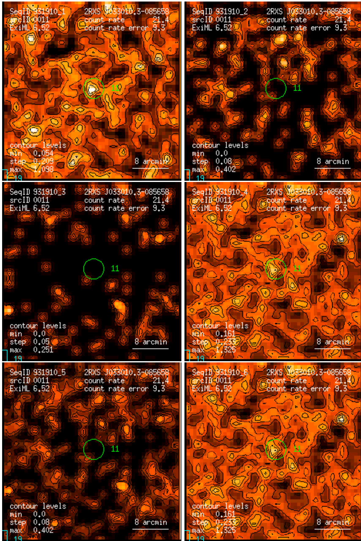
Figure 11: RASS 931910: detection 0011: band rate images, Gaussian filter: (1) PSPC channels 11 – 41, (2) 52 – 90, (3) 91 – 201, (4) 11 – 235, (5) 52 – 201, (6) 11 – 201. Broad band rates in counts/ks. Band rate contour levels in counts/ks/arcmin 2 .
