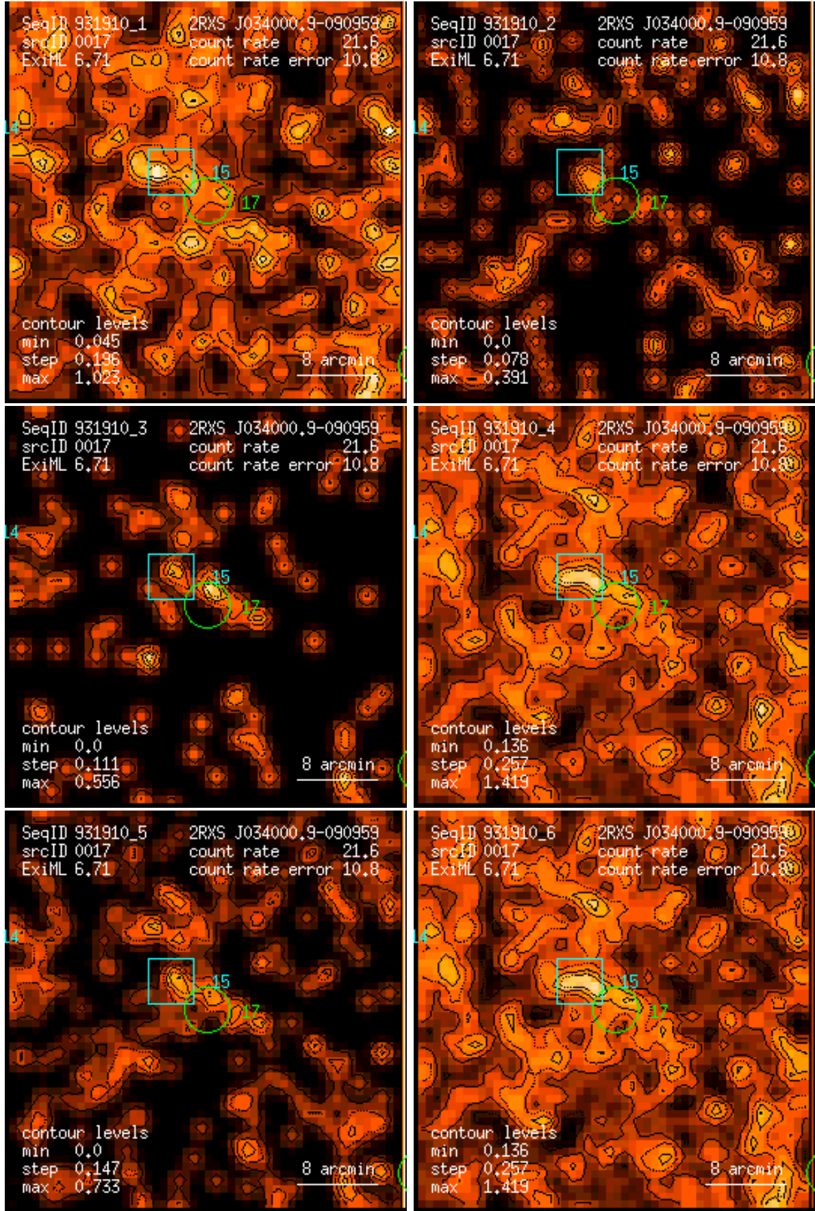
Figure 17: RASS 931910: detection 0017: band rate images, Gaussian filter: (1) PSPC channels 11 – 41, (2) 52 – 90, (3) 91 – 201, (4) 11 – 235, (5) 52 – 201, (6) 11 – 201. Broad band rates in counts/ks. Band rate contour levels in counts/ks/arcmin 2 .
