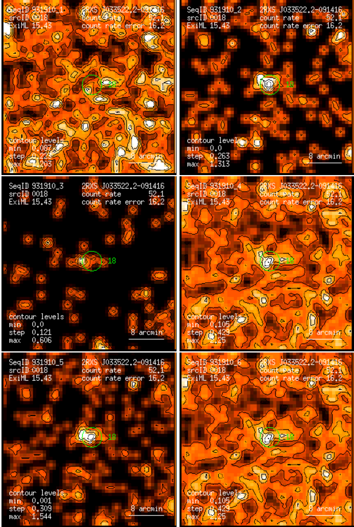
Figure 18: RASS 931910: detection 0018: band rate images, Gaussian filter: (1) PSPC channels 11 – 41, (2) 52 – 90, (3) 91 – 201, (4) 11 – 235, (5) 52 – 201, (6) 11 – 201. Broad band rates in counts/ks. Band rate contour levels in counts/ks/arcmin 2 .
