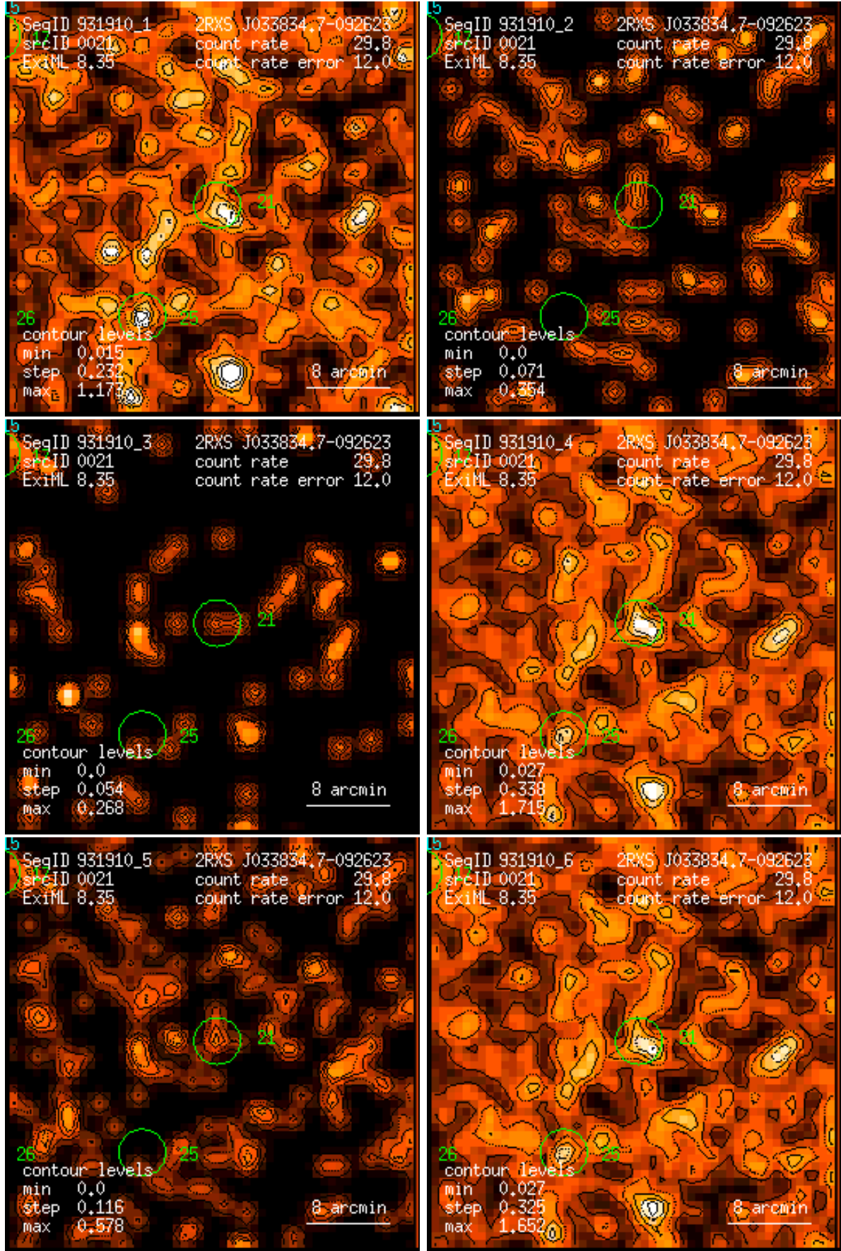
Figure 21: RASS 931910: detection 0021: band rate images, Gaussian filter: (1) PSPC channels 11 – 41, (2) 52 – 90, (3) 91 – 201, (4) 11 – 235, (5) 52 – 201, (6) 11 – 201. Broad band rates in counts/ks. Band rate contour levels in counts/ks/arcmin 2 .
