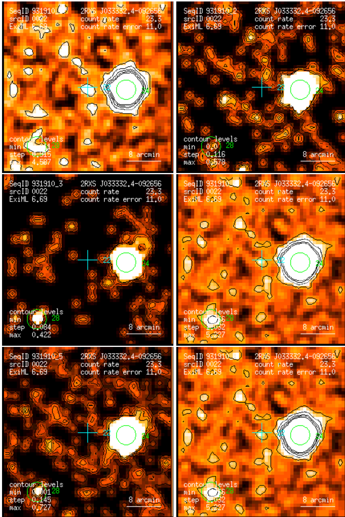
Figure 22: RASS 931910: detection 0022: band rate images, Gaussian filter: (1) PSPC channels 11 – 41, (2) 52 – 90, (3) 91 – 201, (4) 11 – 235, (5) 52 – 201, (6) 11 – 201. Broad band rates in counts/ks. Band rate contour levels in counts/ks/arcmin 2 .
