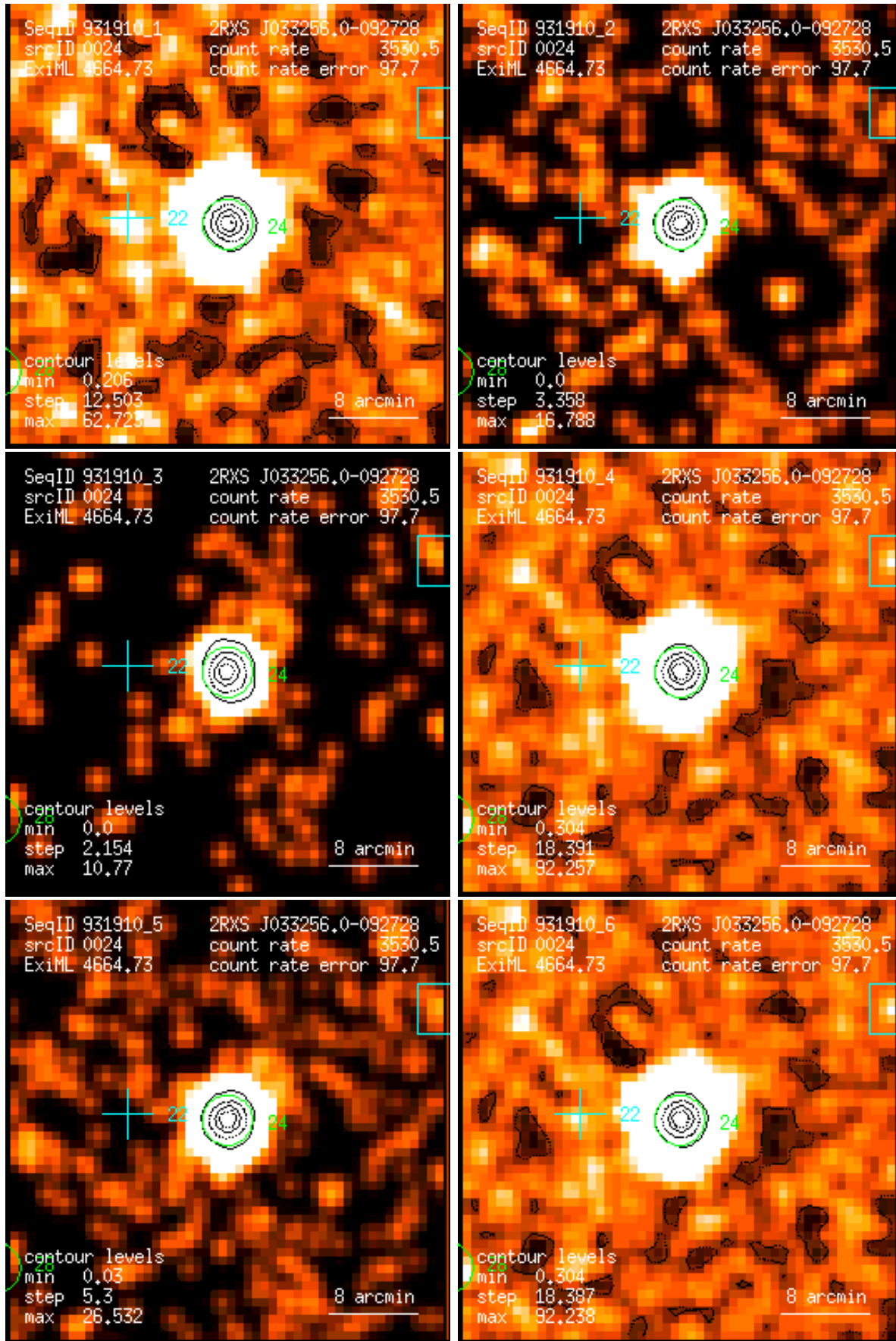
Figure 24: RASS 931910: detection 0024: band rate images, Gaussian filter: (1) PSPC channels 11 – 41, (2) 52 – 90, (3) 91 – 201, (4) 11 – 235, (5) 52 – 201, (6) 11 – 201. Broad band rates in counts/ks. Band rate contour levels in counts/ks/arcmin 2 .
