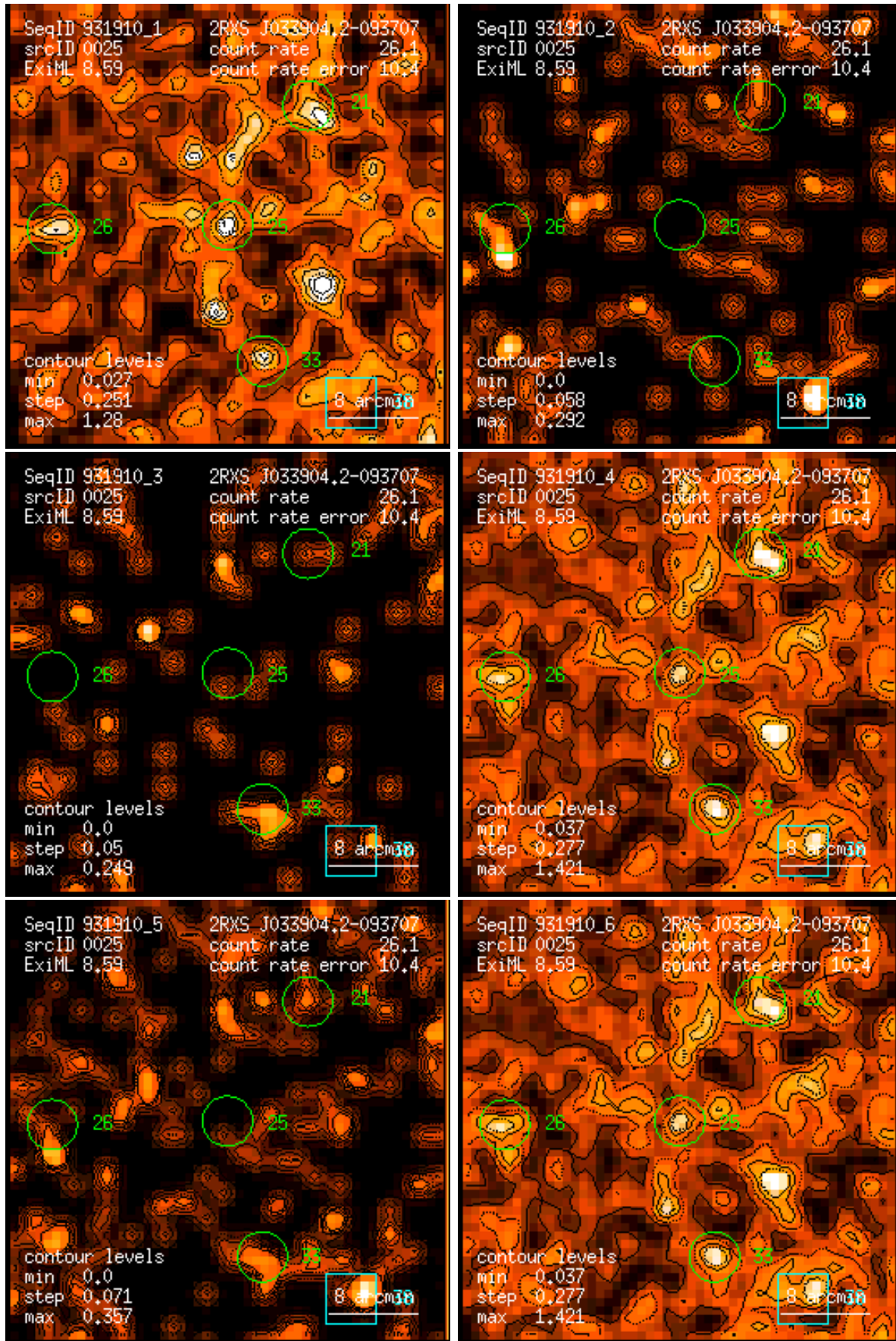
Figure 25: RASS 931910: detection 0025: band rate images, Gaussian filter: (1) PSPC channels 11 – 41, (2) 52 – 90, (3) 91 – 201, (4) 11 – 235, (5) 52 – 201, (6) 11 – 201. Broad band rates in counts/ks. Band rate contour levels in counts/ks/arcmin 2 .
