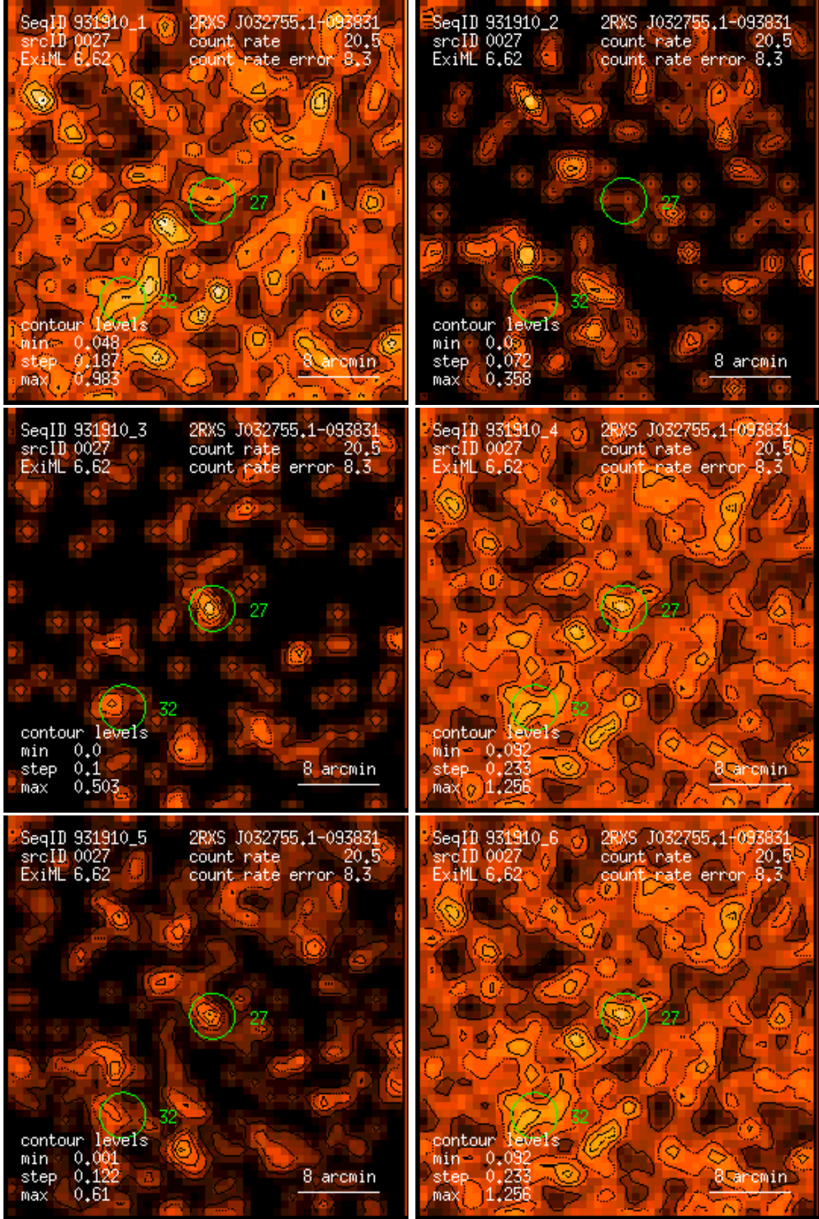
Figure 27: RASS 931910: detection 0027: band rate images, Gaussian filter: (1) PSPC channels 11 – 41, (2) 52 – 90, (3) 91 – 201, (4) 11 – 235, (5) 52 – 201, (6) 11 – 201. Broad band rates in counts/ks. Band rate contour levels in counts/ks/arcmin 2 .
