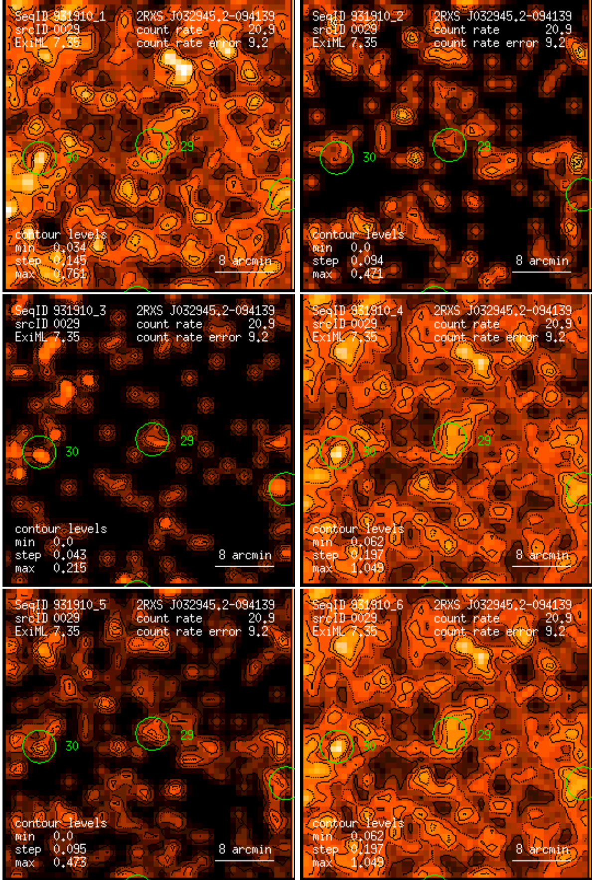
Figure 29: RASS 931910: detection 0029: band rate images, Gaussian filter: (1) PSPC channels 11 – 41, (2) 52 – 90, (3) 91 – 201, (4) 11 – 235, (5) 52 – 201, (6) 11 – 201. Broad band rates in counts/ks. Band rate contour levels in counts/ks/arcmin 2 .
