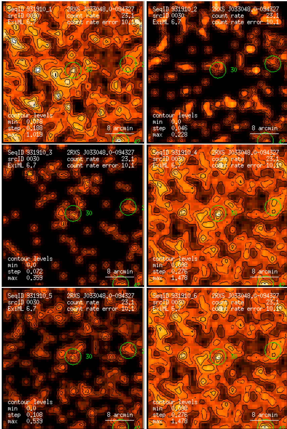
Figure 30: RASS 931910: detection 0030: band rate images, Gaussian filter: (1) PSPC channels 11 – 41, (2) 52 – 90, (3) 91 – 201, (4) 11 – 235, (5) 52 – 201, (6) 11 – 201. Broad band rates in counts/ks. Band rate contour levels in counts/ks/arcmin 2 .
