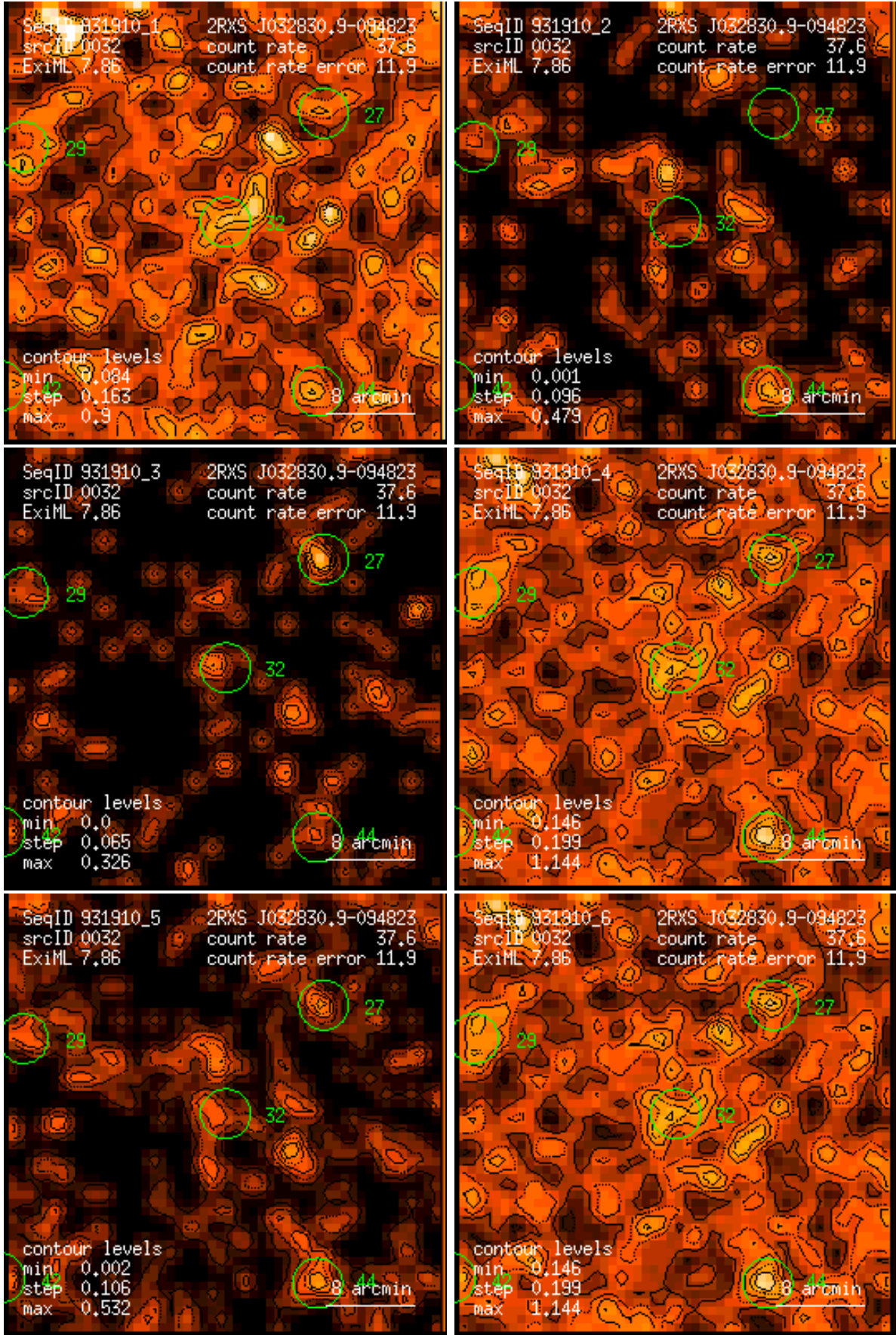
Figure 32: RASS 931910: detection 0032: band rate images, Gaussian filter: (1) PSPC channels 11 – 41, (2) 52 – 90, (3) 91 – 201, (4) 11 – 235, (5) 52 – 201, (6) 11 – 201. Broad band rates in counts/ks. Band rate contour levels in counts/ks/arcmin 2 .
