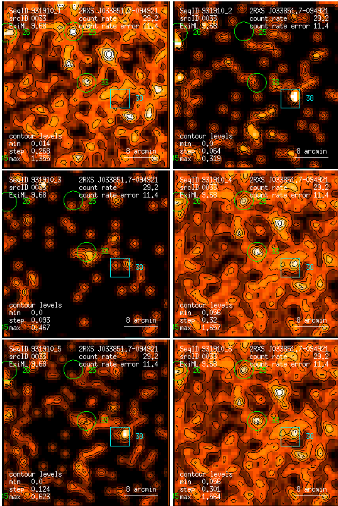
Figure 33: RASS 931910: detection 0033: band rate images, Gaussian filter: (1) PSPC channels 11 – 41, (2) 52 – 90, (3) 91 – 201, (4) 11 – 235, (5) 52 – 201, (6) 11 – 201. Broad band rates in counts/ks. Band rate contour levels in counts/ks/arcmin 2 .
