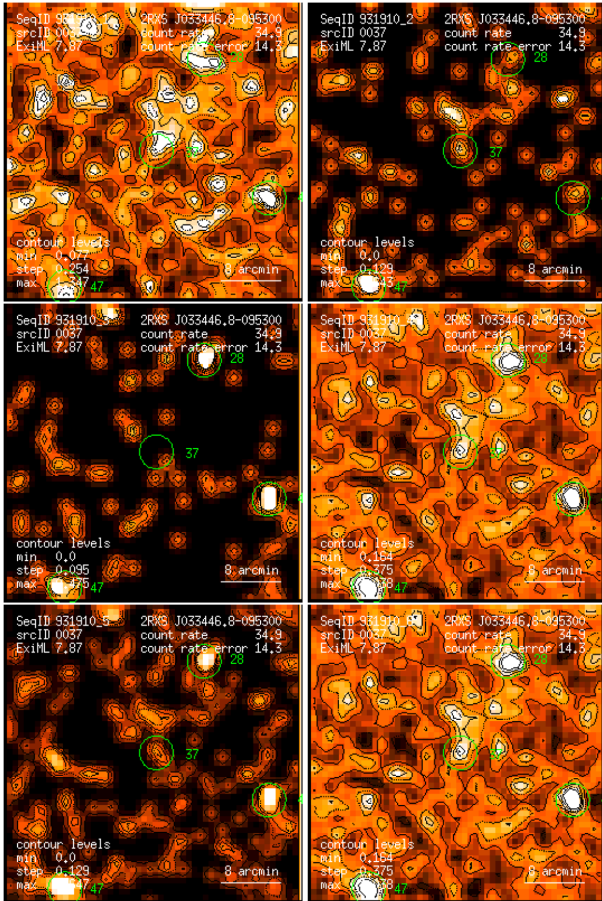
Figure 37: RASS 931910: detection 0037: band rate images, Gaussian filter: (1) PSPC channels 11 – 41, (2) 52 – 90, (3) 91 – 201, (4) 11 – 235, (5) 52 – 201, (6) 11 – 201. Broad band rates in counts/ks. Band rate contour levels in counts/ks/arcmin 2 .
