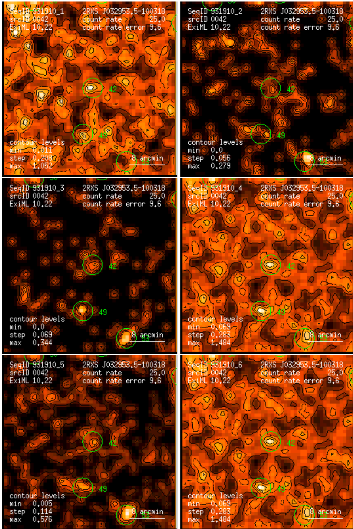
Figure 42: RASS 931910: detection 0042: band rate images, Gaussian filter: (1) PSPC channels 11 – 41, (2) 52 – 90, (3) 91 – 201, (4) 11 – 235, (5) 52 – 201, (6) 11 – 201. Broad band rates in counts/ks. Band rate contour levels in counts/ks/arcmin 2 .
